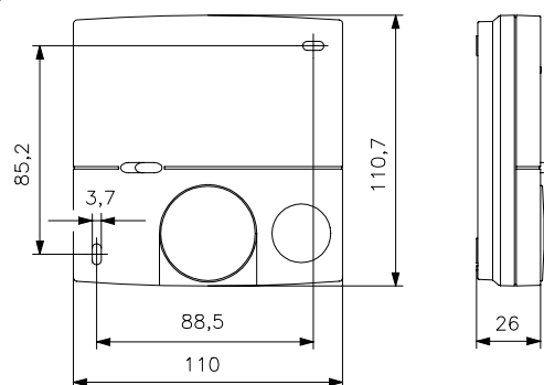
FHY with insert frame
