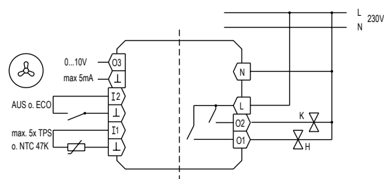
KTRRUu application example – 4-pipe system (230-V version)
