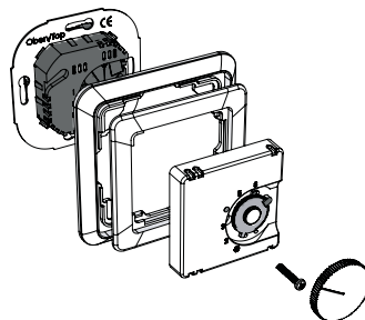
with 50x50 insert frame
