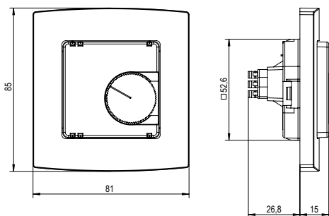
RTBSU with alre frame 'Berlin' (RTBSU-401.xxx#21 types)
