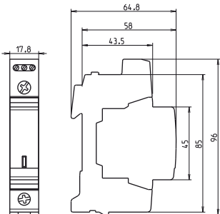
OVR T2 40-275 P TS OVR T2 40-275s P TS OVR T2 70-275s P TS
