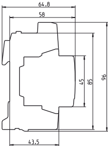
OVR T2 2L 15-75 P TS
