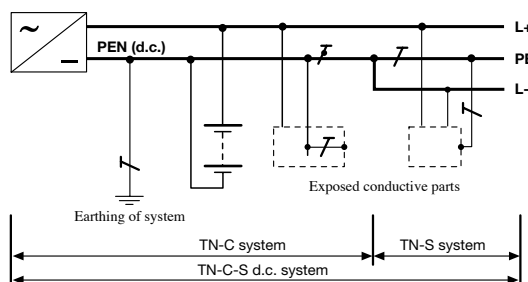
Figure 14 TN C-S d.c. distribution system
