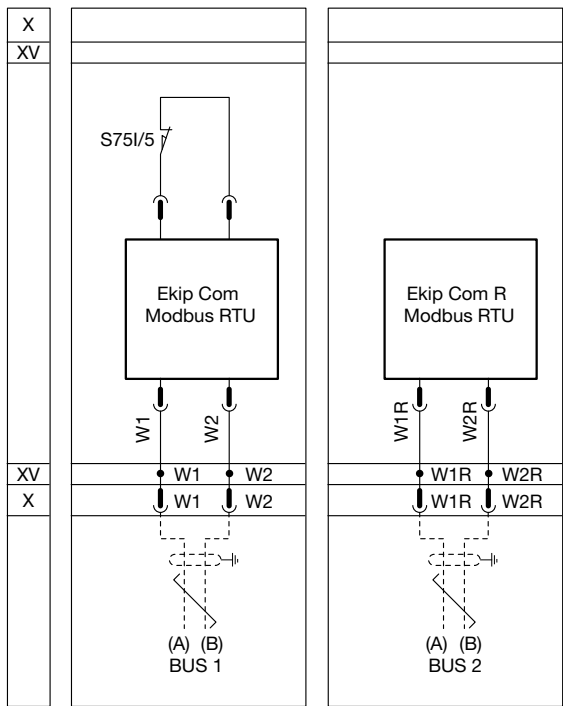
Wiring diagram
