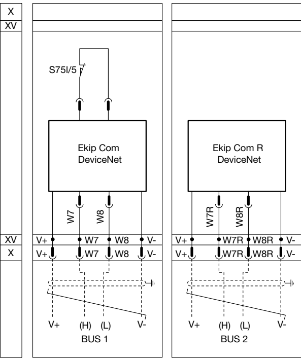
Wiring diagram
