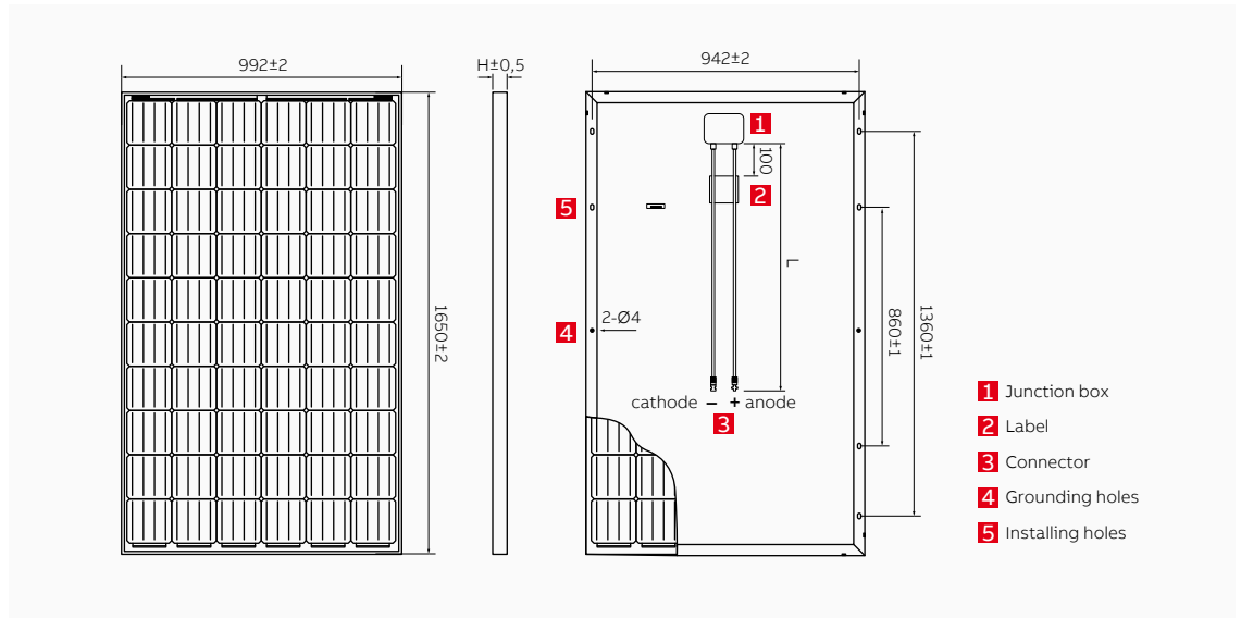
Figure 86 dimensions of the selected module type
