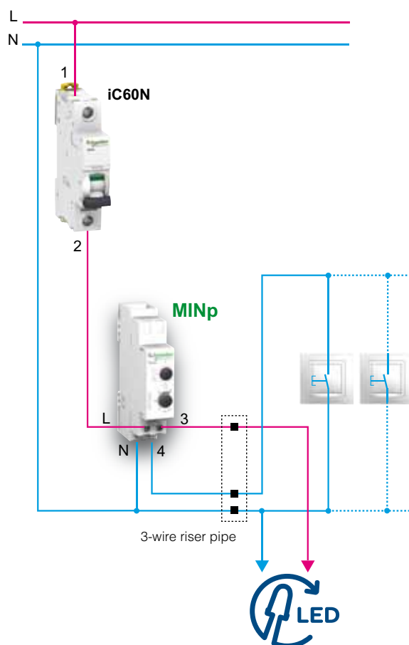
Connection to 3-conductor riser pipe
