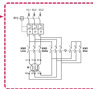
Star-delta starting:
