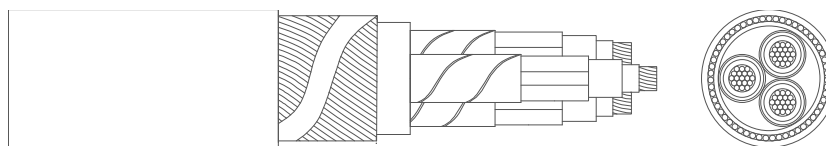
X-VOLT® RHVhMVh 3,6/6 kV
