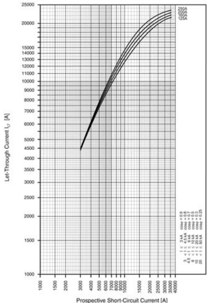
Let-through current BZM2
