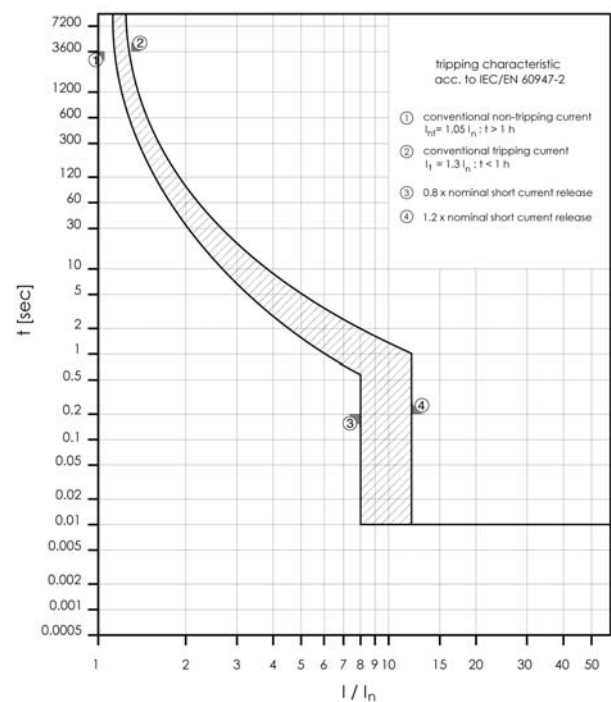
Tripping Curve BZM1 40A, 3-pole
