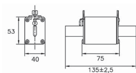
Size 1
