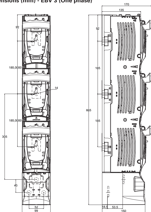
M12 Screws
