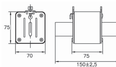
Size 3
