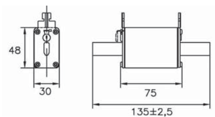
Size 01
