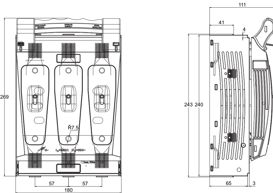
Screw terminals
