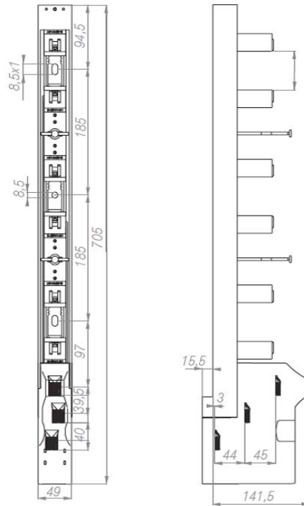
V-Terminals
