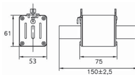
Size 2
