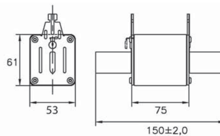
Size 03
