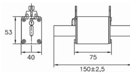
Size 02
