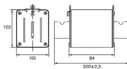
Size 4
