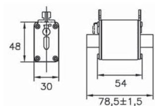
Size 00
