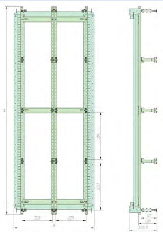
Support Rack XVTL-TG for XVTL...-IVS
