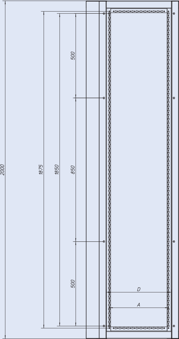
XVTL-CF-./. Corner Frame
