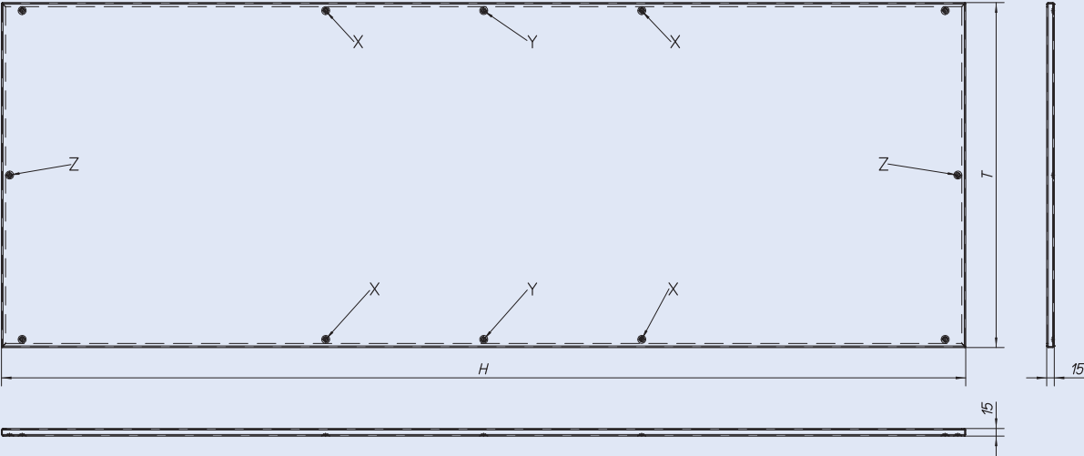
XVTL-PV Separation Panel (galvanised)
