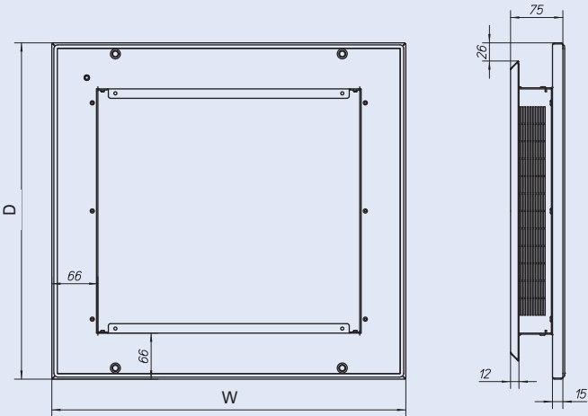
XAD Top Cover
