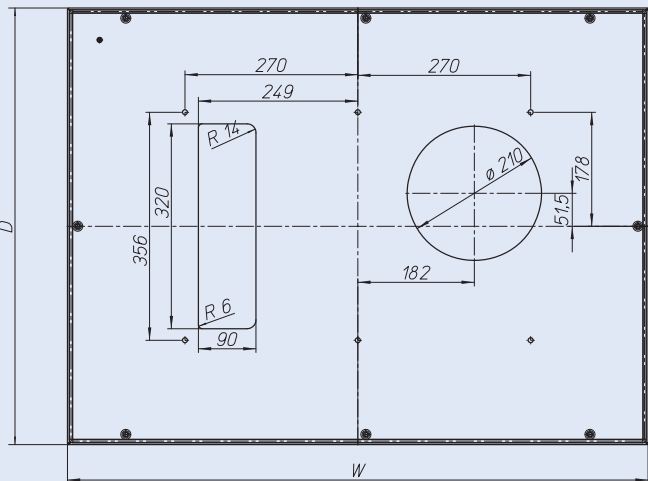
XVTL-MP/T/AC../. Top Cover with cut-outs prepared for air conditioners
