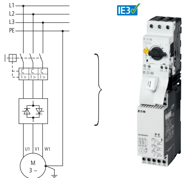
Fig. 9: motor feeder, soft starter DS7, in-line configuration, combined with PKZM0
