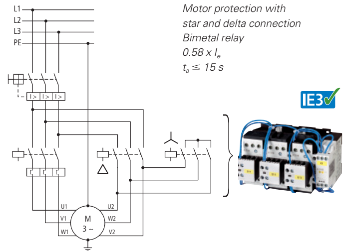
Fig. 8: motor feeder, star-delta starter, cw rotation, example of SDAINL
