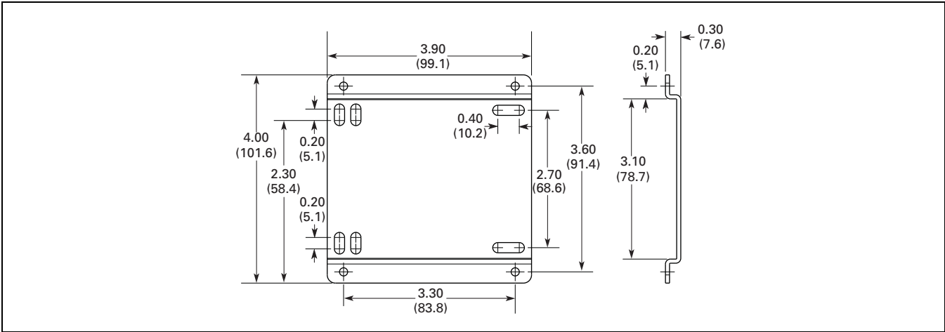
Figure 4.2-1. C441 Motor Insight Conversion Plate
