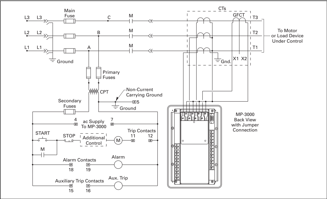
Figure 4.2-4. MP-3000 Wiring
