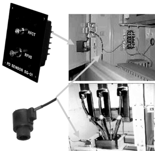
Typical Installation of RFCT Sensor
