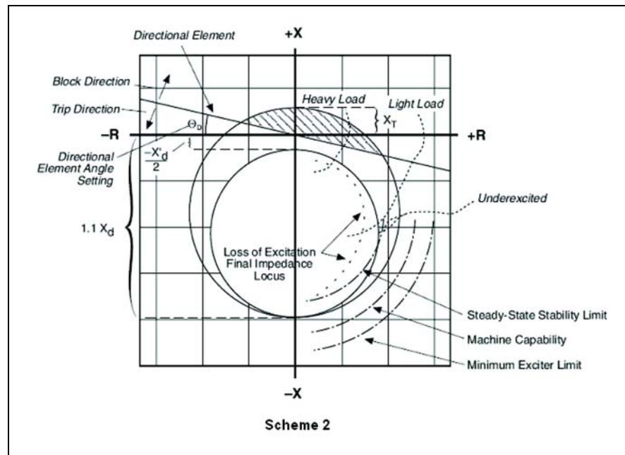
Figure 4.3-13. Scheme 2
