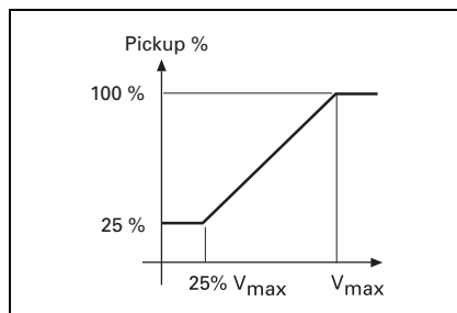
Figure 4.1-24. Voltage Restraint Coil Pickup Characteristics
