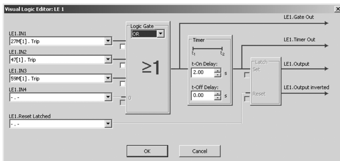
Figure 4.2-9. Visual Logic Editor
