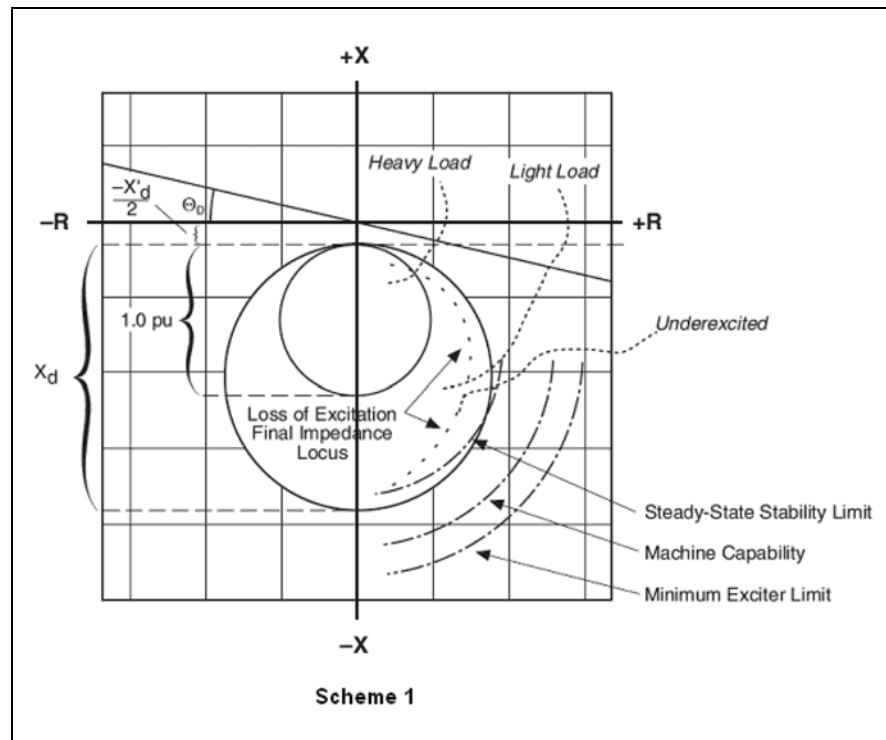
Figure 4.3-12. Scheme 1
