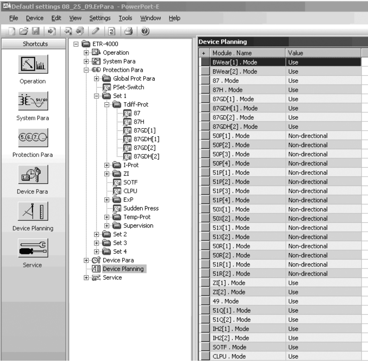
Figure 4.3-1. ETR-4000 Device Planning
