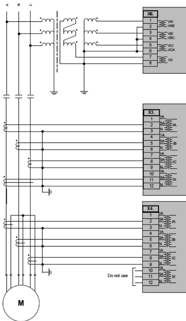
Figure 4.2-15. Typical AC Connections. Wye VTs, 5A CTs, and Ground Current Measured by Residual Connection
