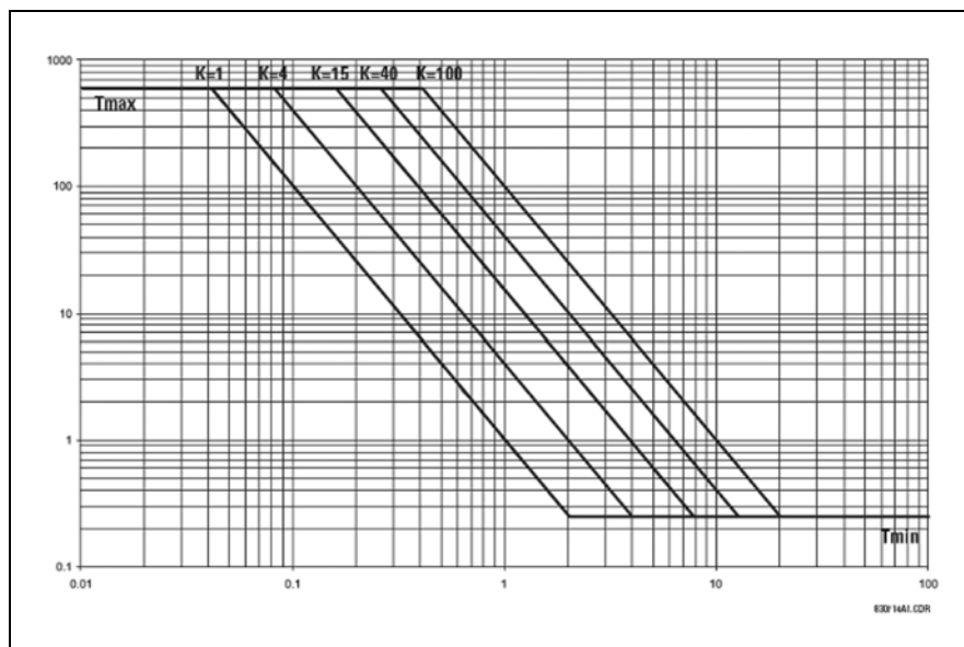
Figure 4.3-11. Overexcitation Protection
