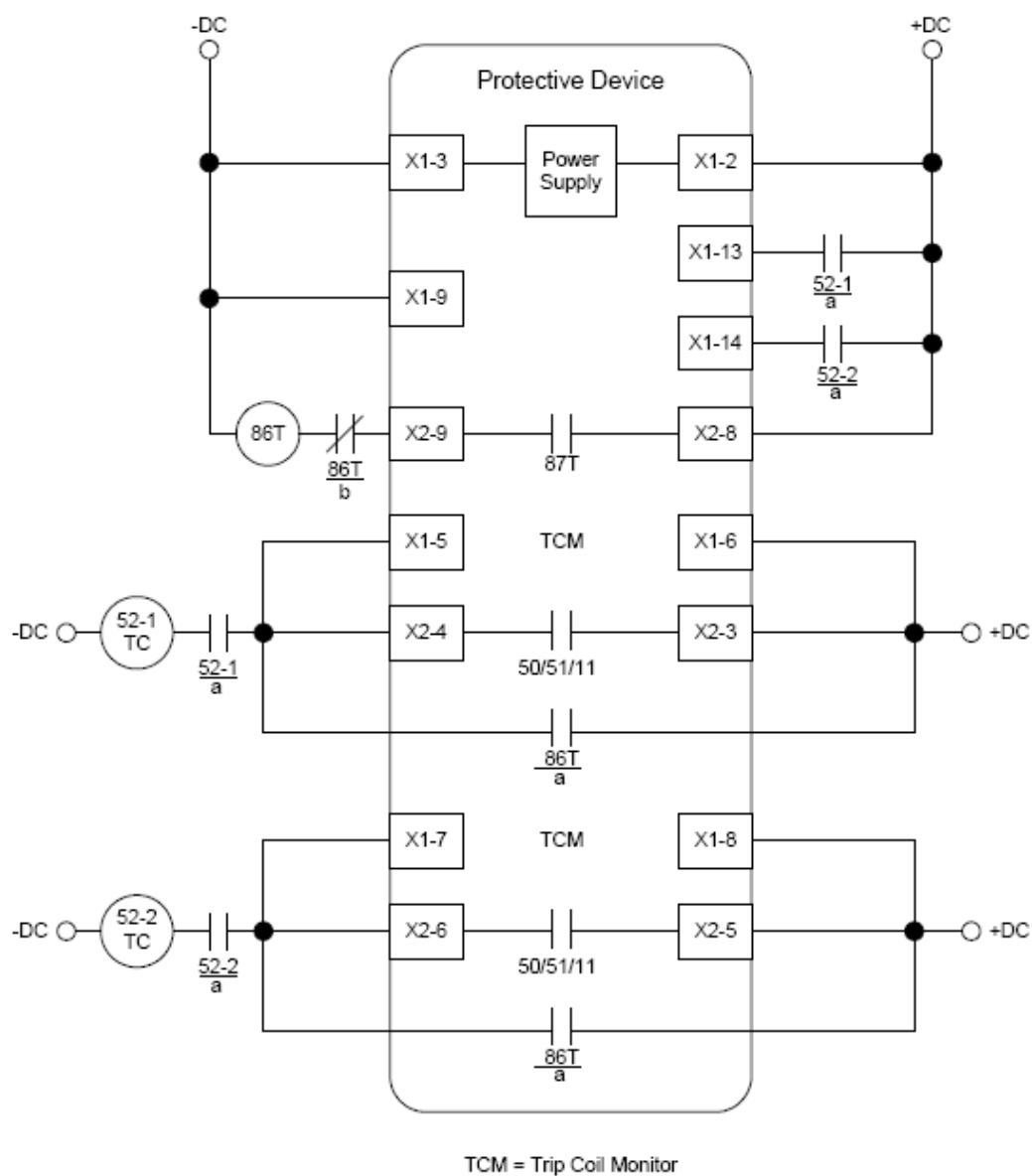
Figure 4.3-8. Typical Control Diagram
