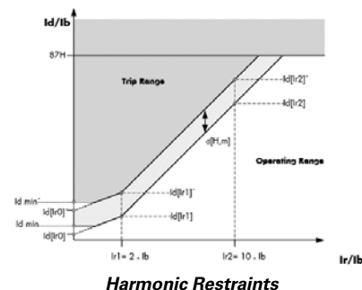
Harmonic Restraints
