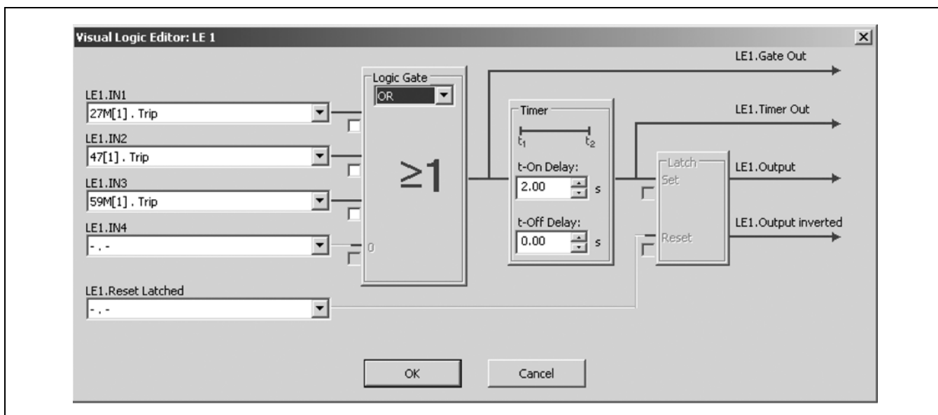
Figure 4.1-25. Visual Logic Editor
