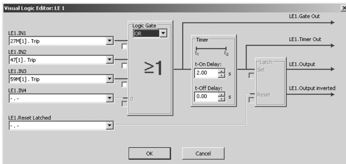
Figure 4.3-14. Visual Logic Editor
