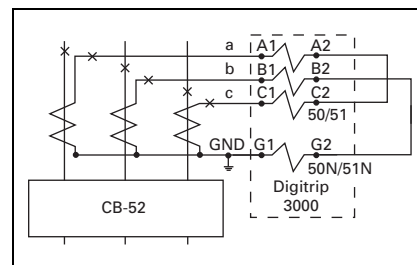
Figure 4.1-4. Residual Ground Connections
