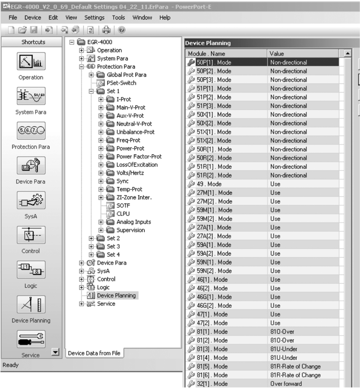
Figure 4.3-19. PowerPort-E EGR-5000 Device Planning
