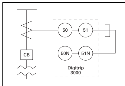
Figure 4.1-2. Transformer Protection
