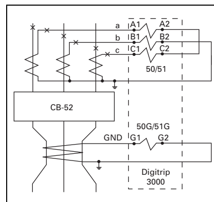
Figure 4.1-5. Separate Zero Sequence Ground CT Connections
