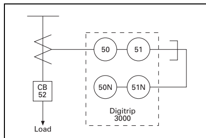
Figure 4.1-1. Primary Feeder Protection
