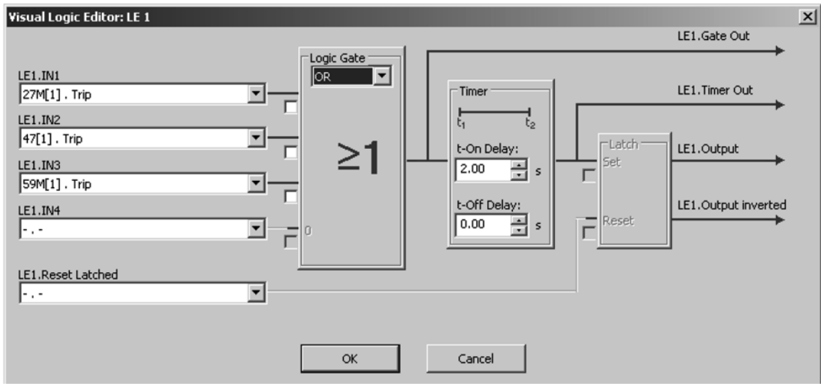
Figure 4.2-13. Programmable Logic
