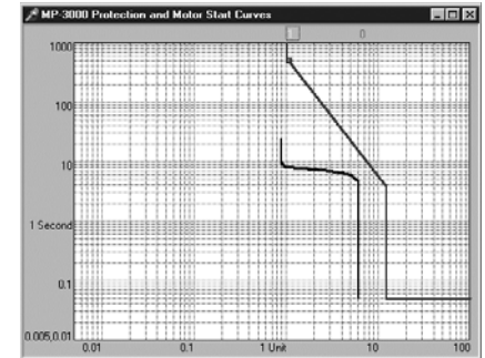
Motor Starting Profile Time/Current Chart
