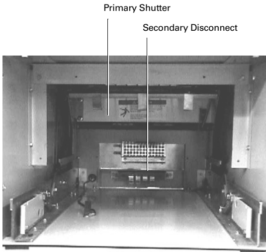
Auxiliary Drawer Compartment
