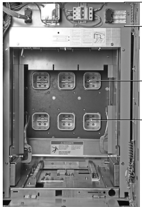
VCP-T Circuit Breaker Compartment (Shutters Shown Open for Illustration)
