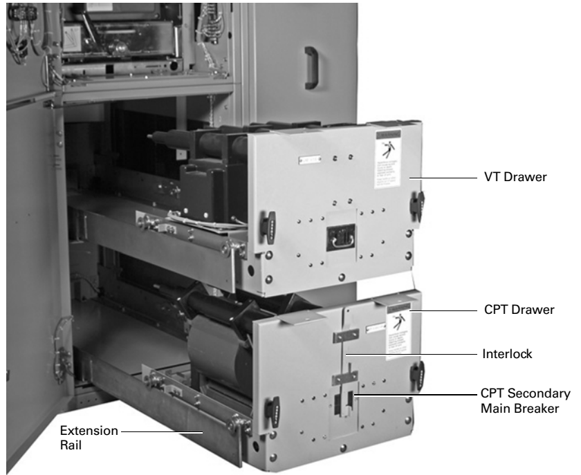
Drawout VT and CPT
