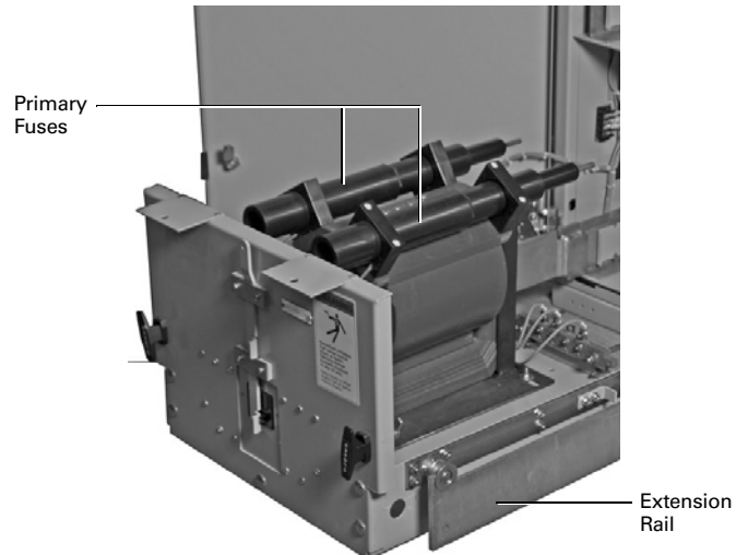
CPT Withdrawn on Extension Rails
