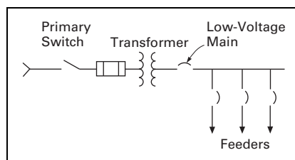
Figure 14.0-1. Simple Radial
