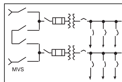
Figure 14.0-4. Loop Selective
