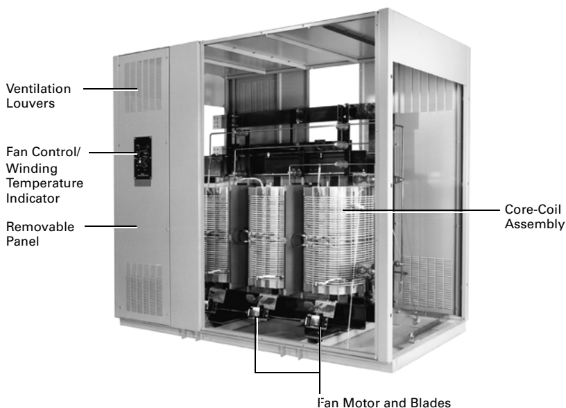
Dry-Type Substation Transformer
