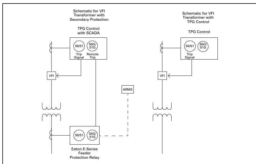
Figure 14.0-7. VFI Schematics with Arcflash Reduction Maintenance System™
