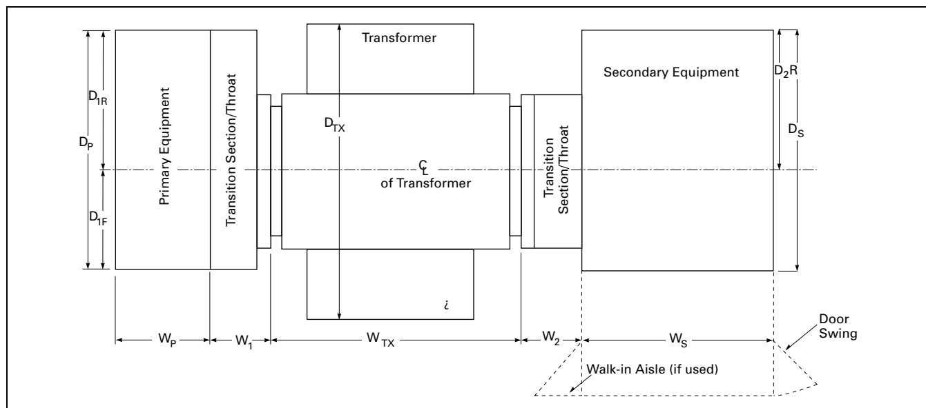
Figure 14.0-10. Liquid-Filled, Outdoor Enclosure—Top View
