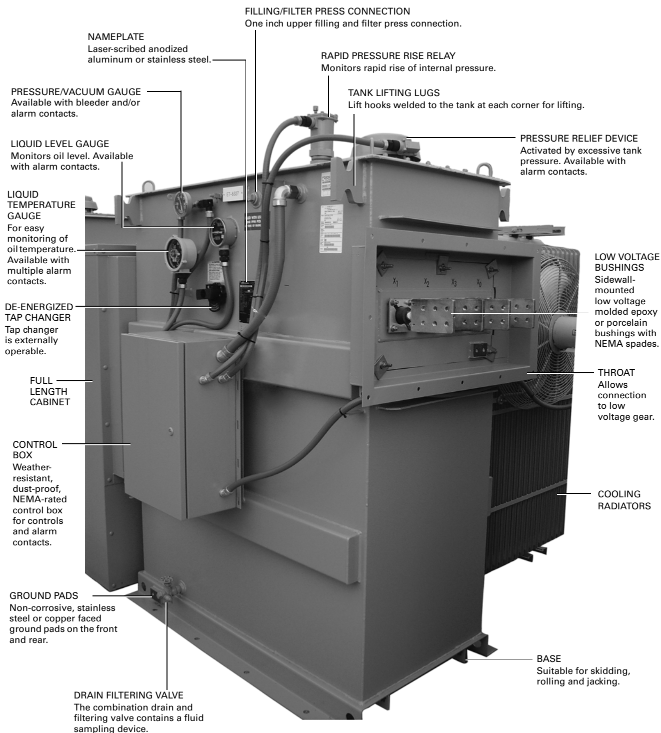
Liquid-Filled Substation Transformer
