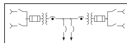
Figure 14.0-5. Spot Network
