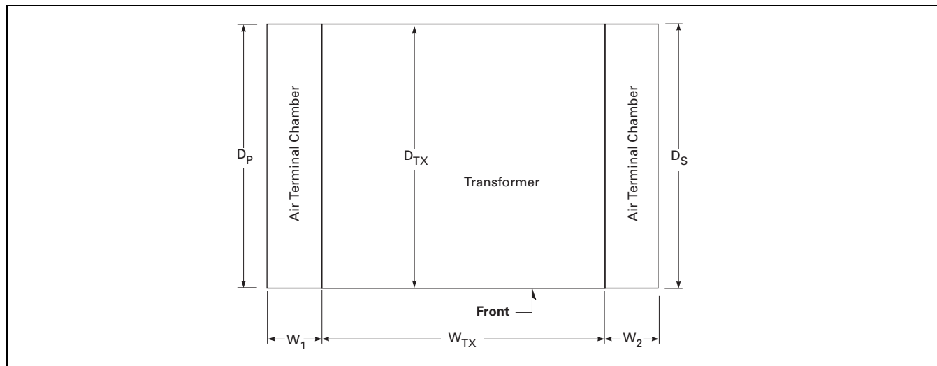
Figure 14.0-14. Dry-Type Indoor/Outdoor Using Air Terminal Chambers—Top View
