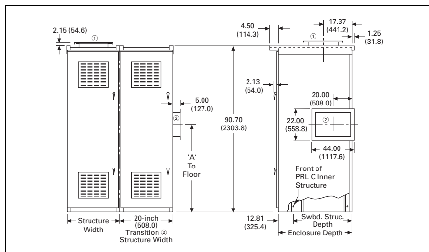
Figure 14.0-21. Front or Rear Access—Non-Walk-in with Flat Roof—Dimensions in Inches (mm)
