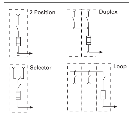
Figure 14.0-6. MVS Switch Arrangements
