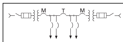
Figure 14.0-3. Secondary Selective
