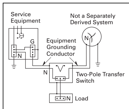
Figure 25.0-6. Non-Separately Derived System
