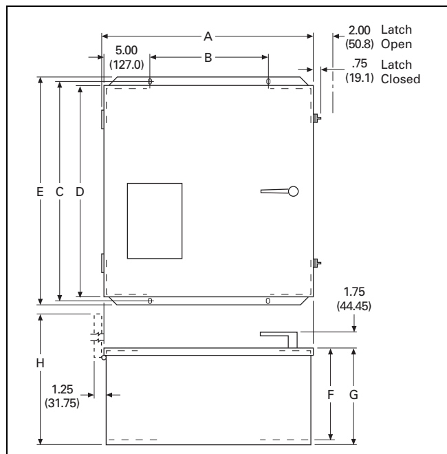
Figure 25.2-1. Dimensions
