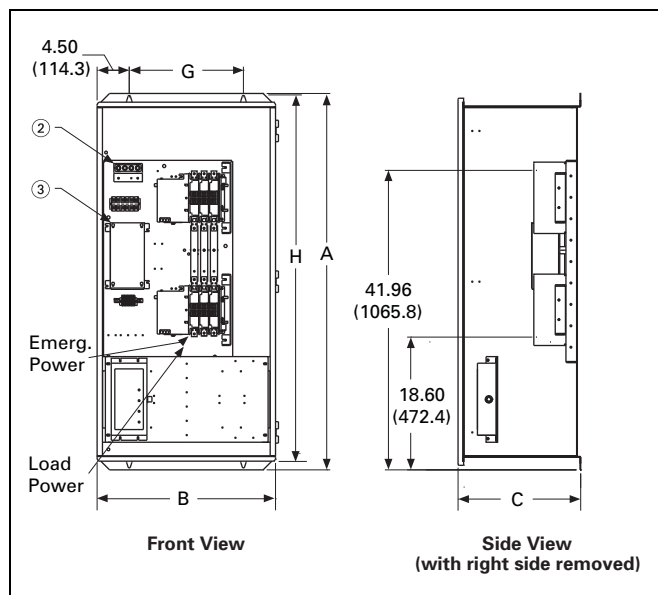
Figure 25.1-11. Automatic Up to 400 A Wallmount NEMA 1
