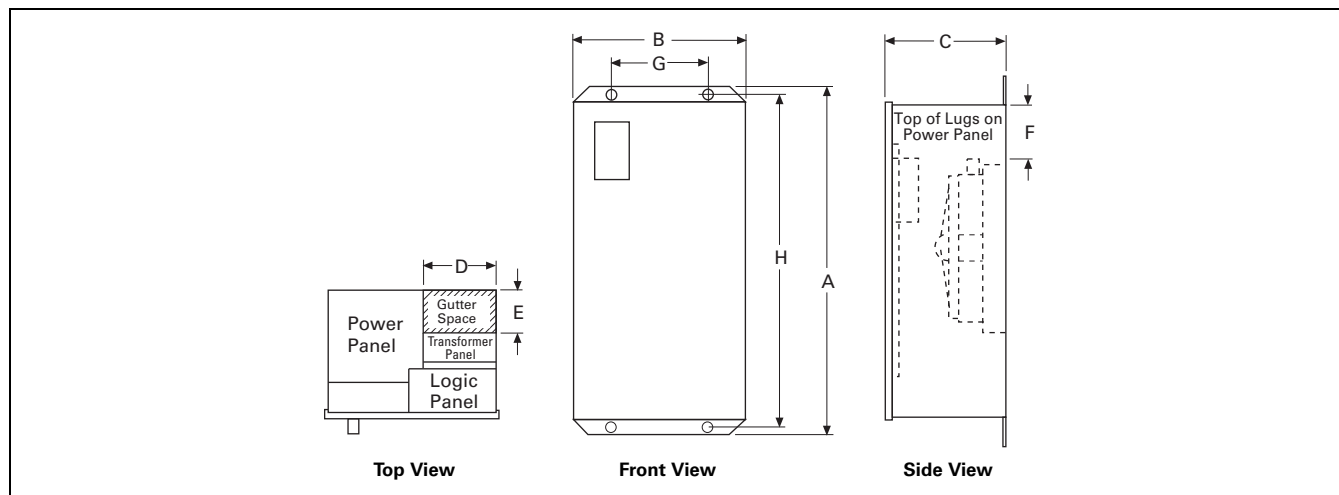
Figure 25.2-4. Dimension Views
