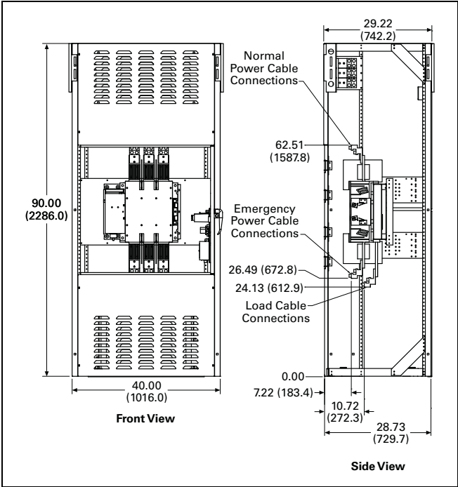
Figure 25.1-9. Automatic, Non-Automatic Open Transition NEMA 1 Enclosure
