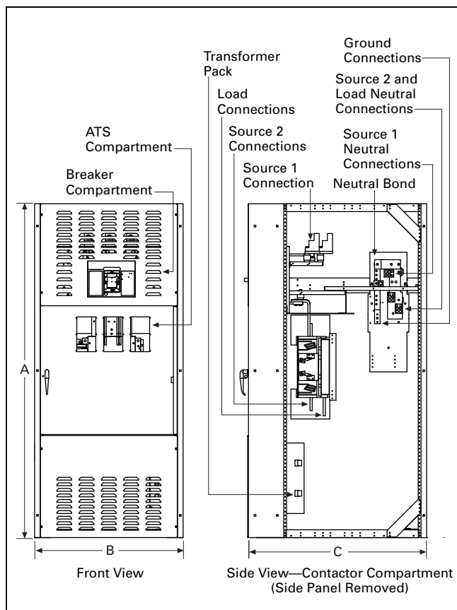
Figure 25.1-23. Automatic, 1200 A and 1600 A, NEMA 1
