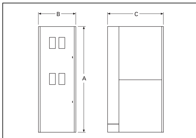
Figure 25.3-3. 200–3200 A Drawout NEMA 1
