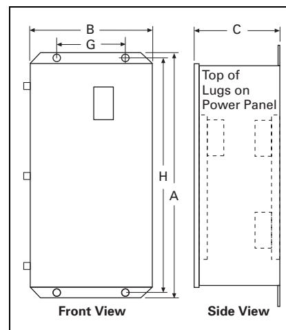
Figure 25.1-8. Automatic, Non-Automatic Up to 400 A Wallmount Outline NEMA1 and NEMA 3R
