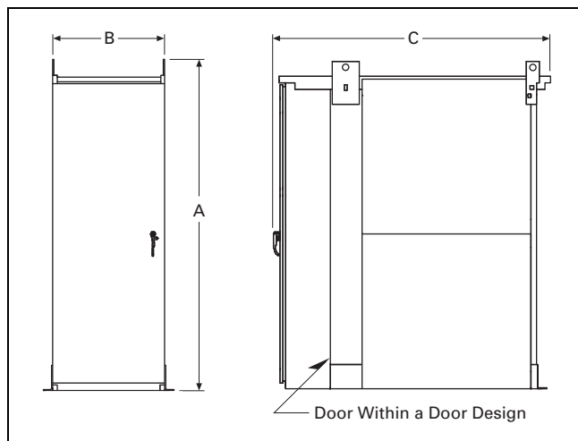
Figure 25.1-24. Automatic 1000–1600 A, NEMA 3R
