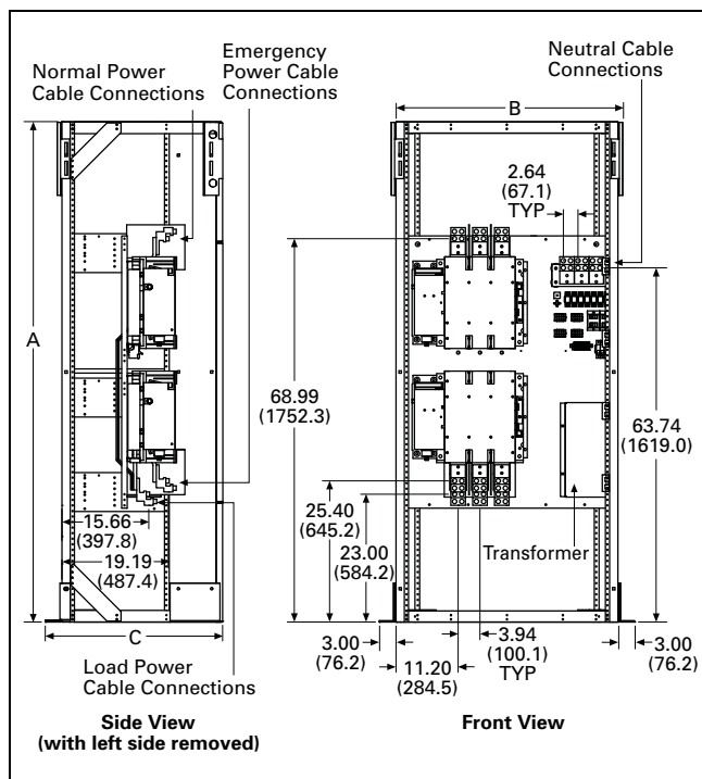
Figure 25.1-12. Automatic 600–1200 A—Floor-Standing NEMA 1
