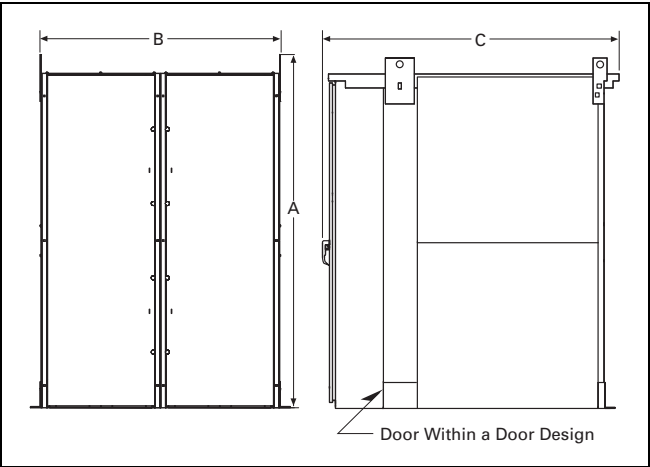
Figure 25.3-9. 200–3200 A Drawout NEMA 3R
