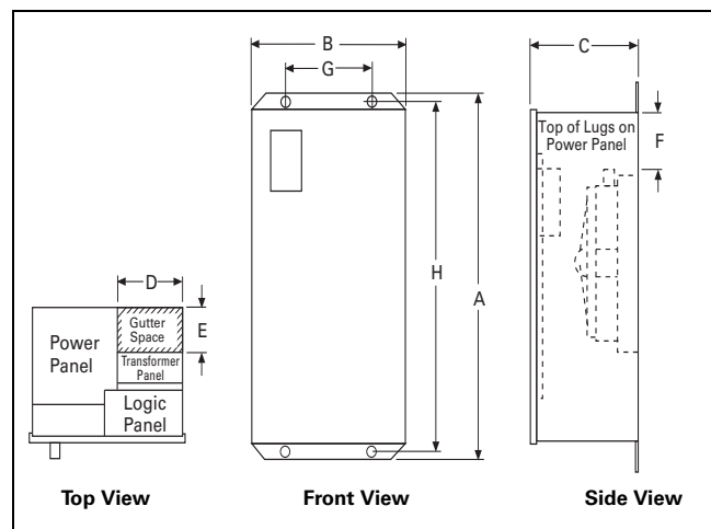
Figure 25.2-2. Dimensions
