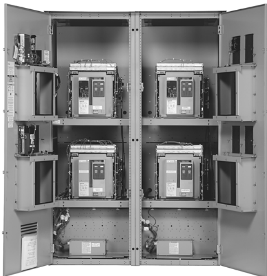
Magnum Bypass Isolation Front View NEMA 1 Through-the-Door
