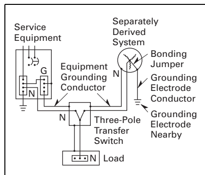
Figure 25.0-5. Separately Derived System
