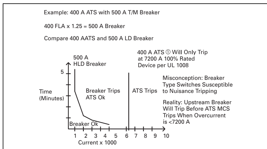
Figure 25.0-4. Built-in Protection
