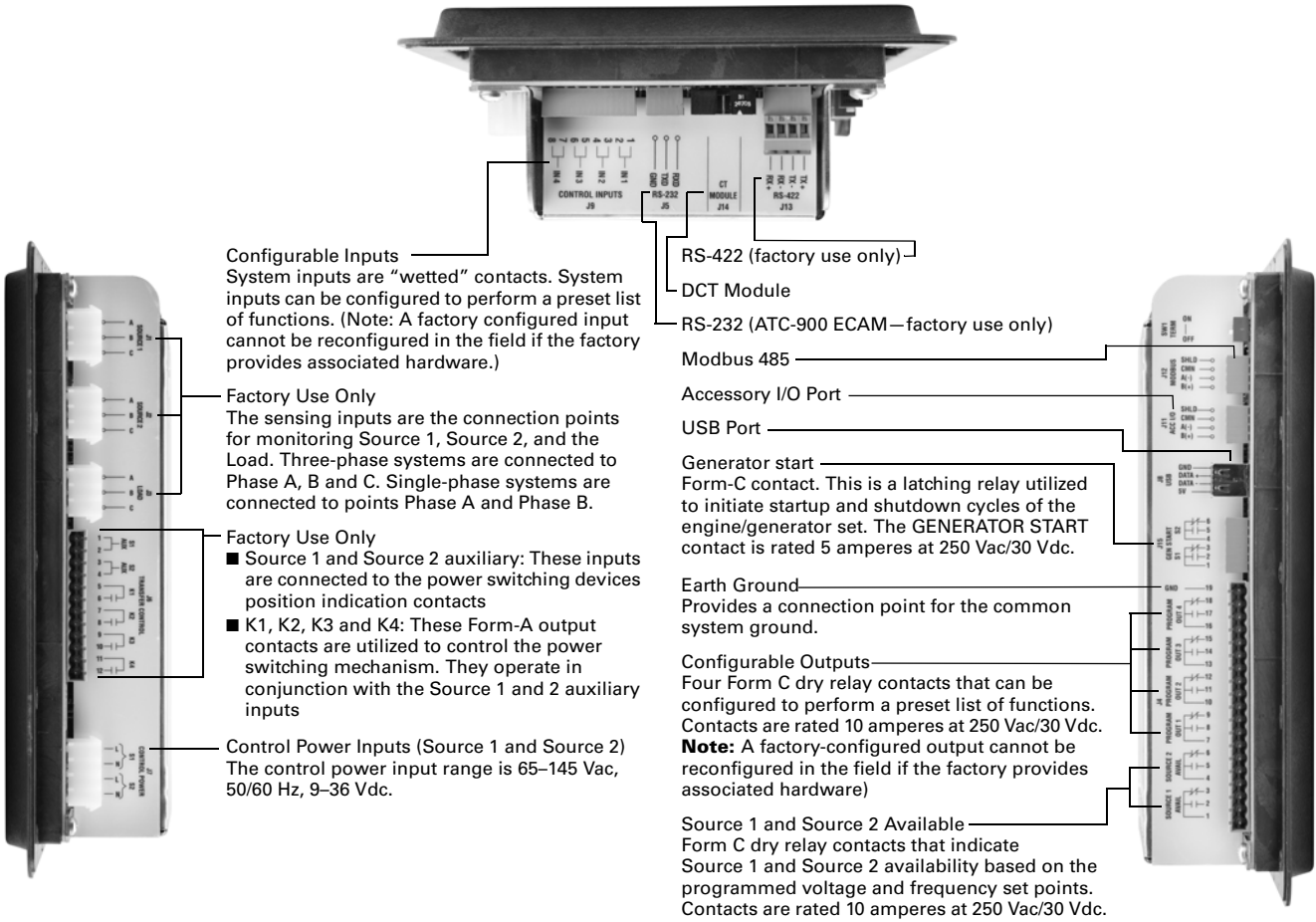
ATC-900 Connections
