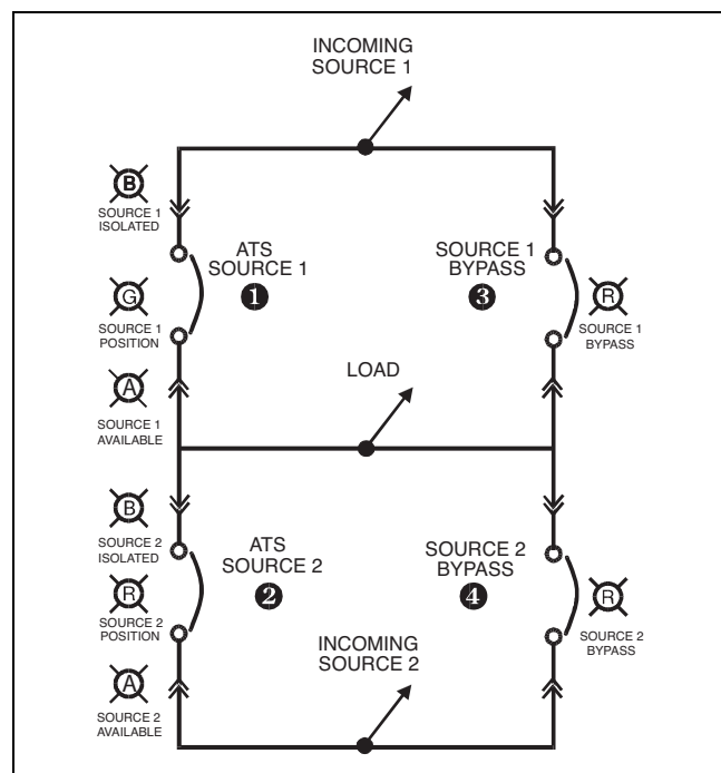
Figure 25.3-7. Typical Bypass Isolation Switch Schematic
