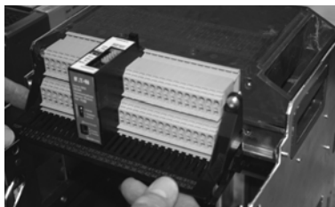
Communication Adapter Module Cassette Mounted in Secondary Terminal Blocks
