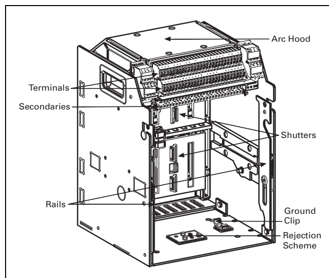
Figure 26.2-2. Cassette/Cradle Components
