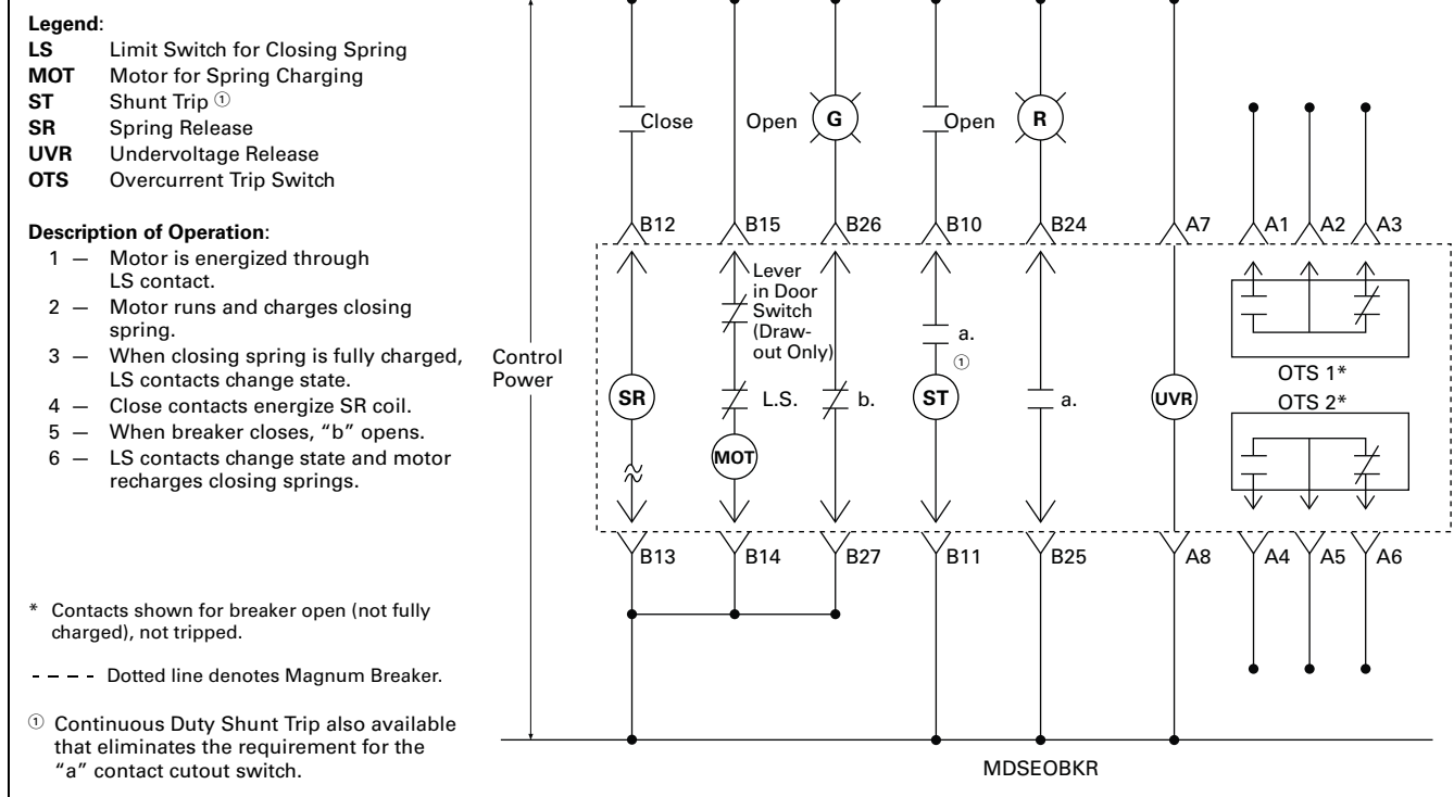
Figure 26.1-9. Typical Magnum Breaker Control Circuit Diagram
