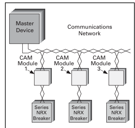
Figure 26.2-3. Communications Adapter Modules in a Modbus RTU, INCOM or PROFIBUS DP Network
