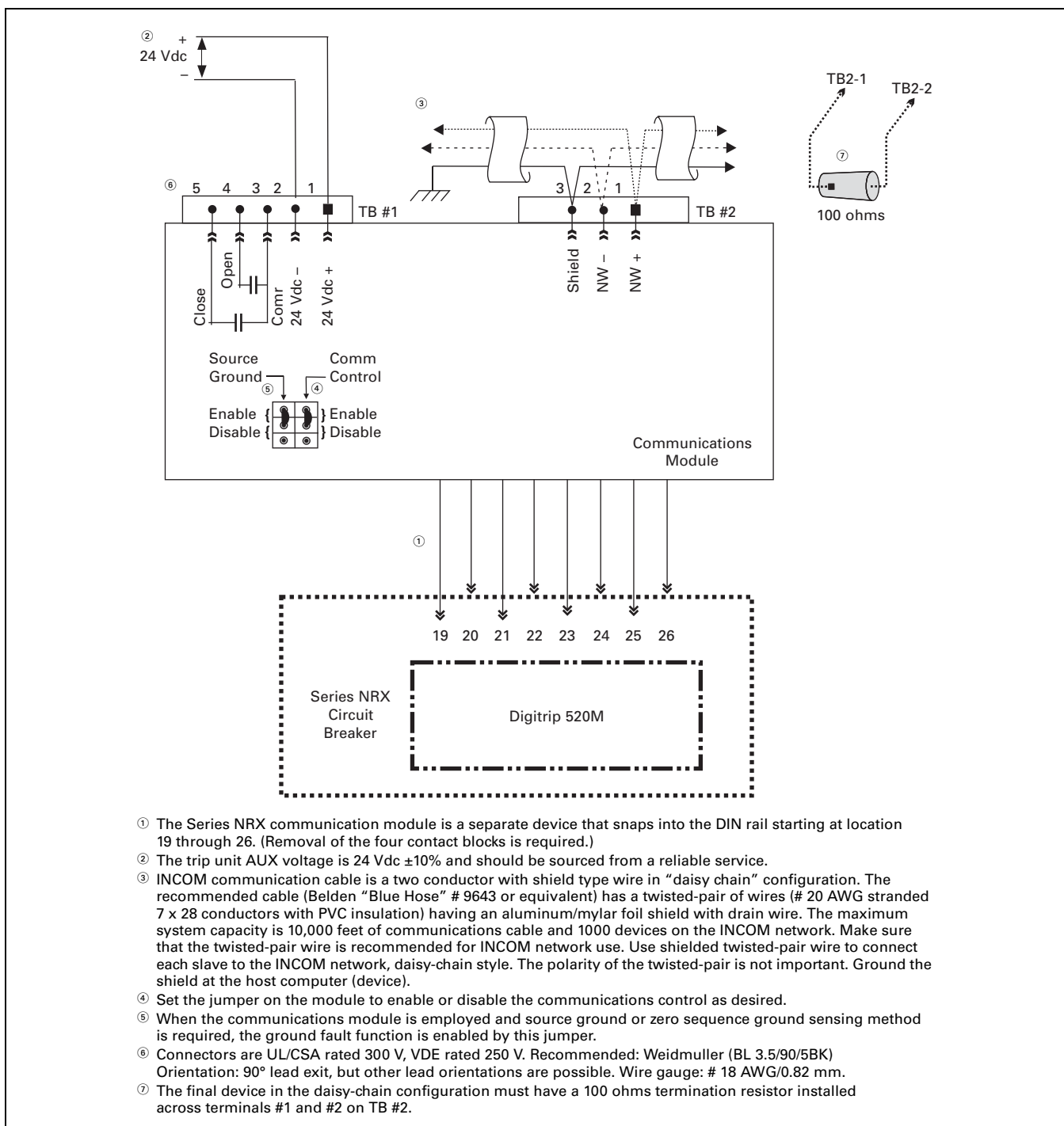
Figure 26.2-6. Series NRX INCOM Communication with Digitrip 520M
