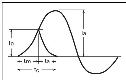
Figure 26.1-2. Current Limiting
