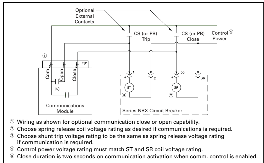
Figure 26.2-4. Communications Control (SR and ST Wiring)
