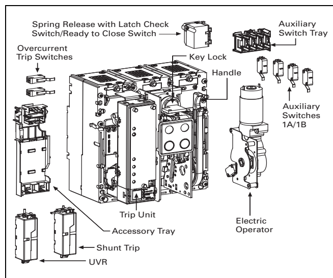
Figure 26.2-1. Breaker and Accessories
