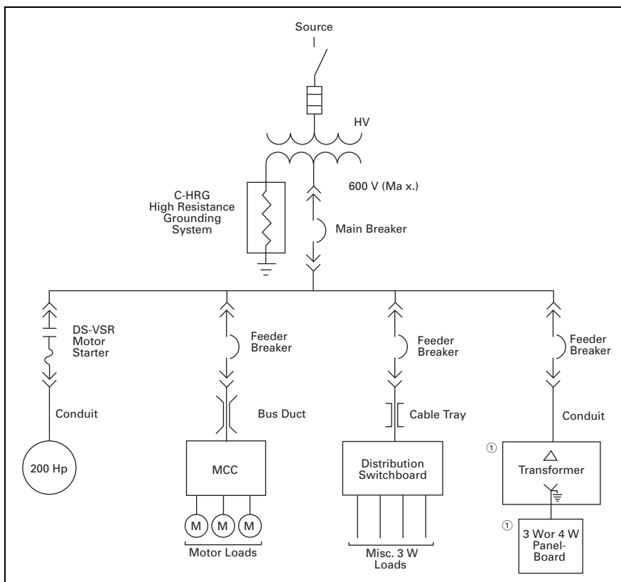
Figure 36.2-1. Typical Distribution System
