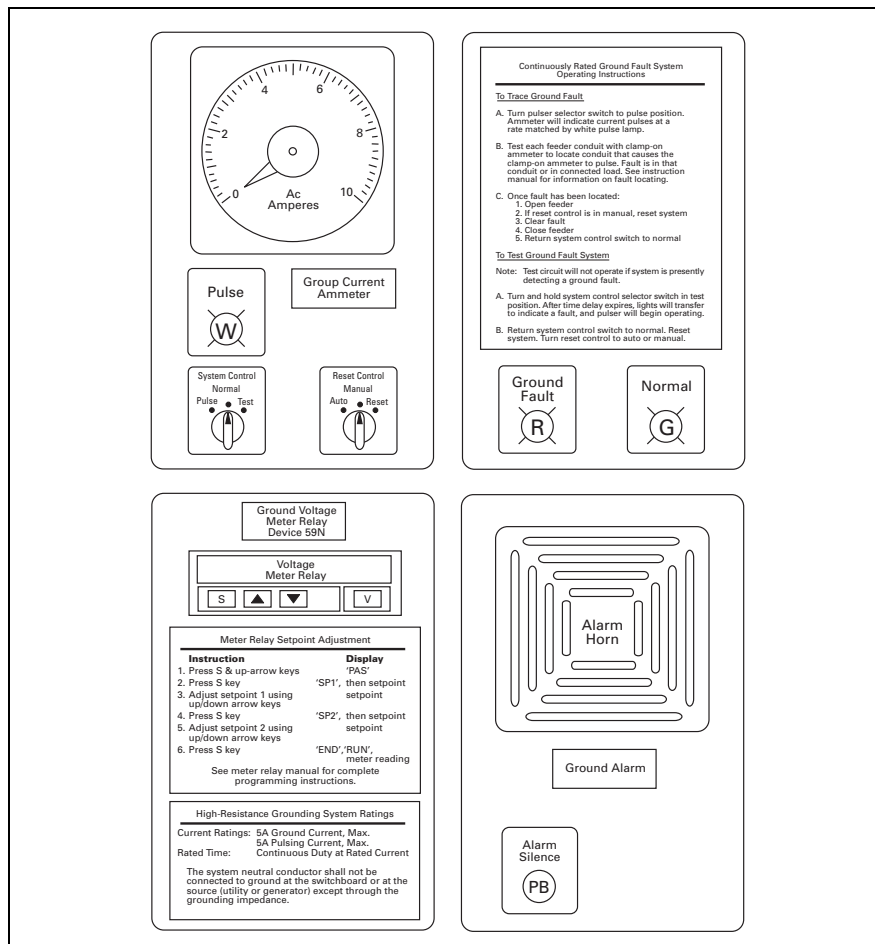
Figure 36.2-2. Front Door Layout
