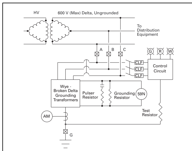
Figure 36.2-8. Three-Wire Source—Fault Detection via Voltmeter Relay
