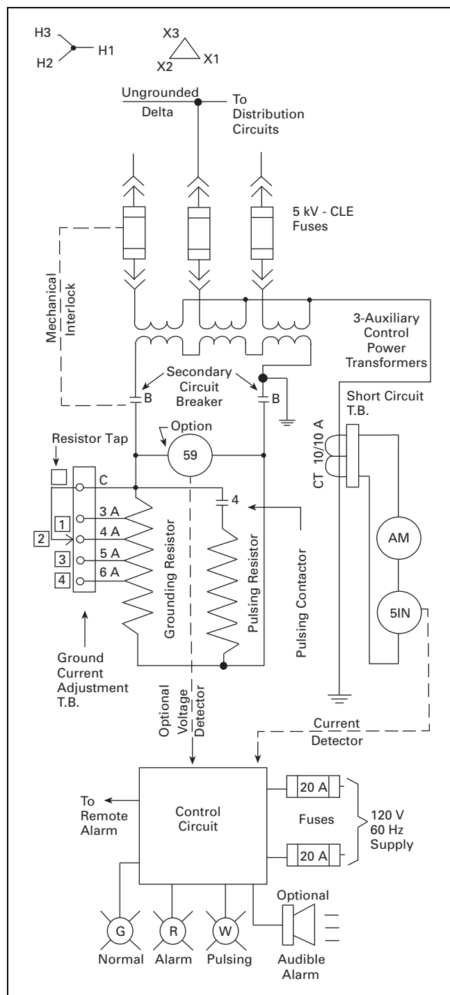
Figure 36.1-3. Ungrounded Delta System (With Standard Current and Optional Voltage Relay Fault Detectors)
