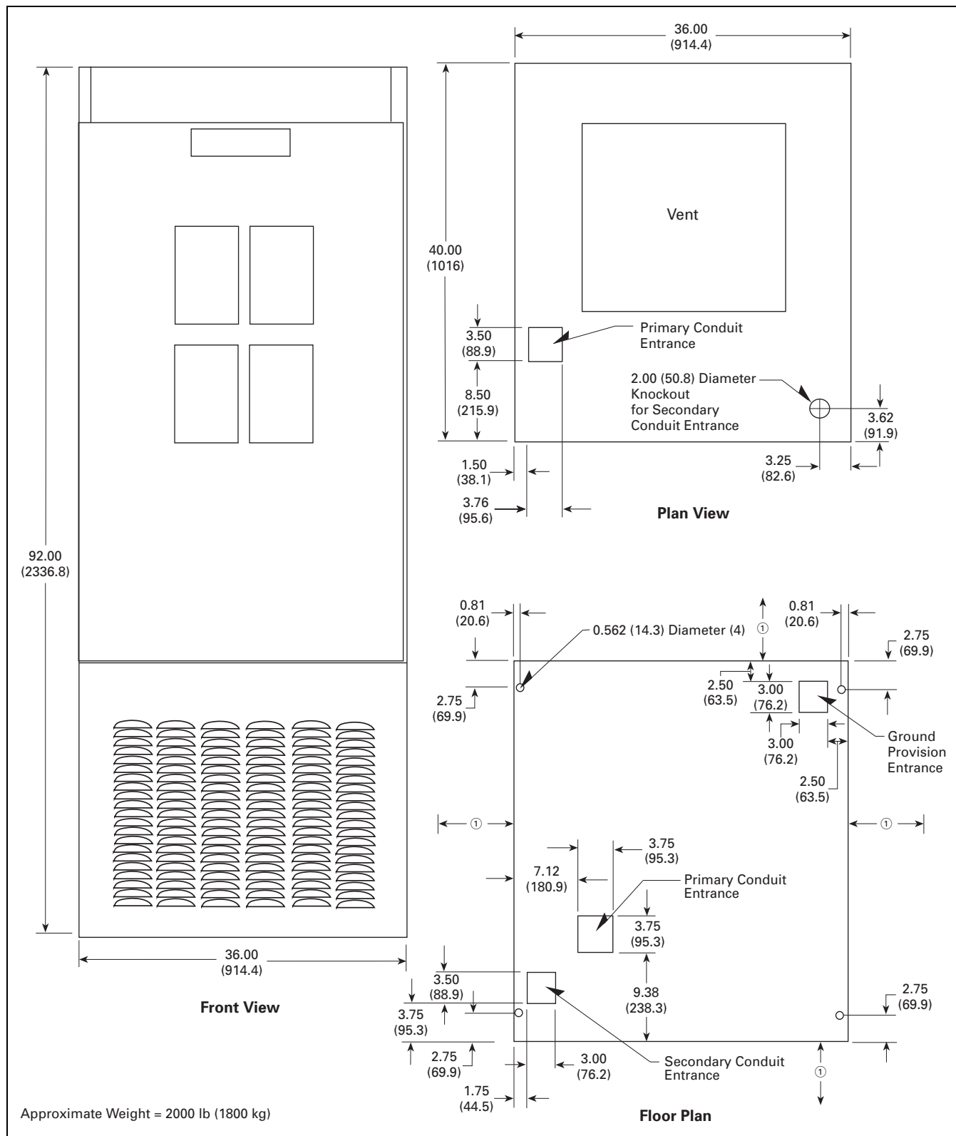
Figure 36.1-4. NEMA 1 Free-Standing
