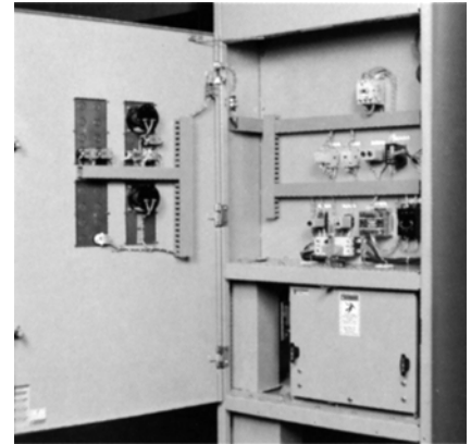
C-HRG Unit Shown with the Door Open
