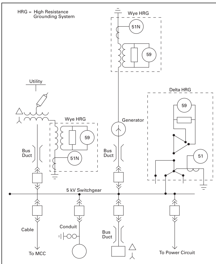
Figure 36.1-1. HRG—High Resistance Grounding System
