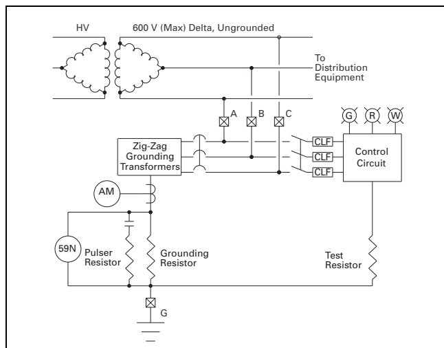
Figure 36.2-6. Three-Wire Source—Fault Detection via Voltmeter Relay
