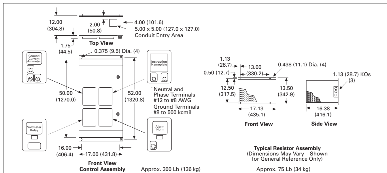
Figure 36.2-11. NEMA 1 Wall Mounted
