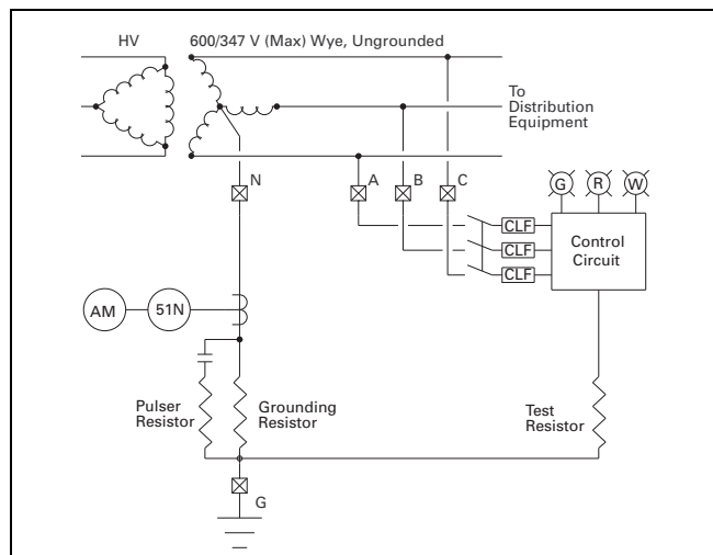
Figure 36.2-3. Four-Wire Source—Fault Detection via Current Relay
