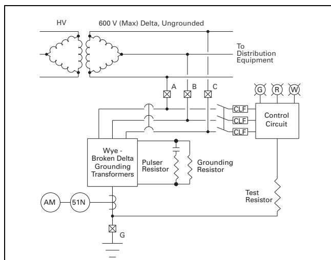
Figure 36.2-7. Three-Wire Source—Fault Detection via Current Relay
