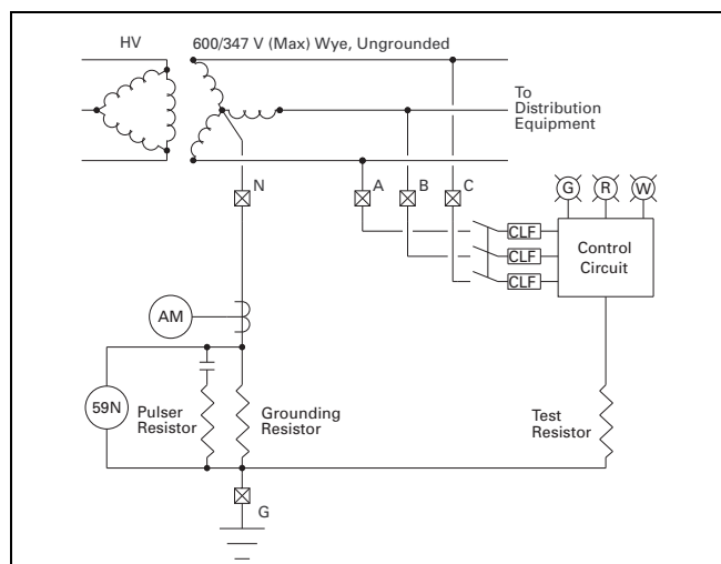
Figure 36.2-4. Four-Wire Source—Fault Detection via Voltmeter Relay
