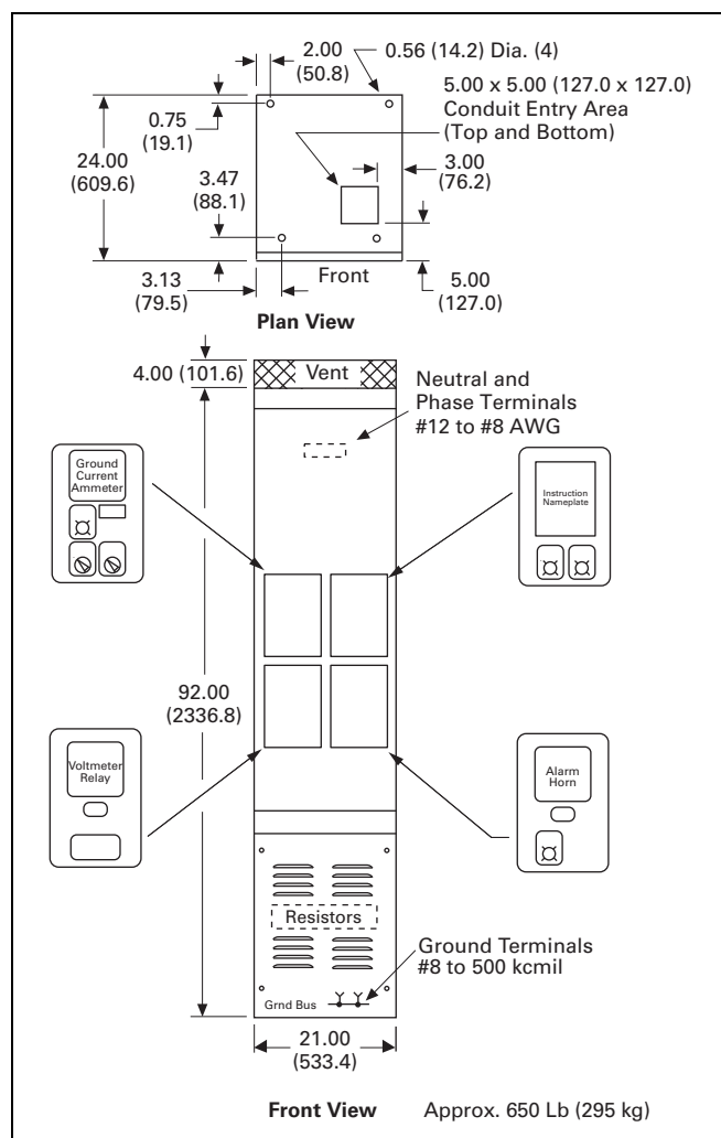
Figure 36.2-9. NEMA 1 Free Standing
