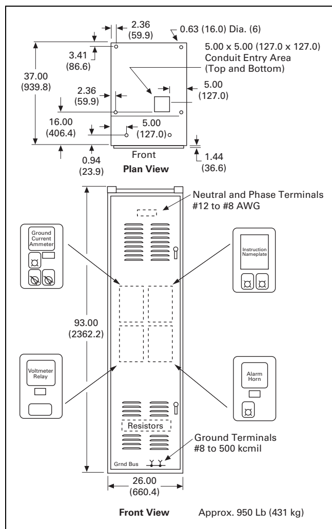
Figure 36.2-10. NEMA 3R Outdoor
