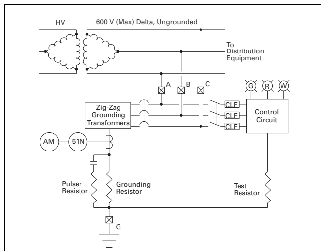
Figure 36.2-5. Three-Wire Source—Fault Detection via Current Relay
