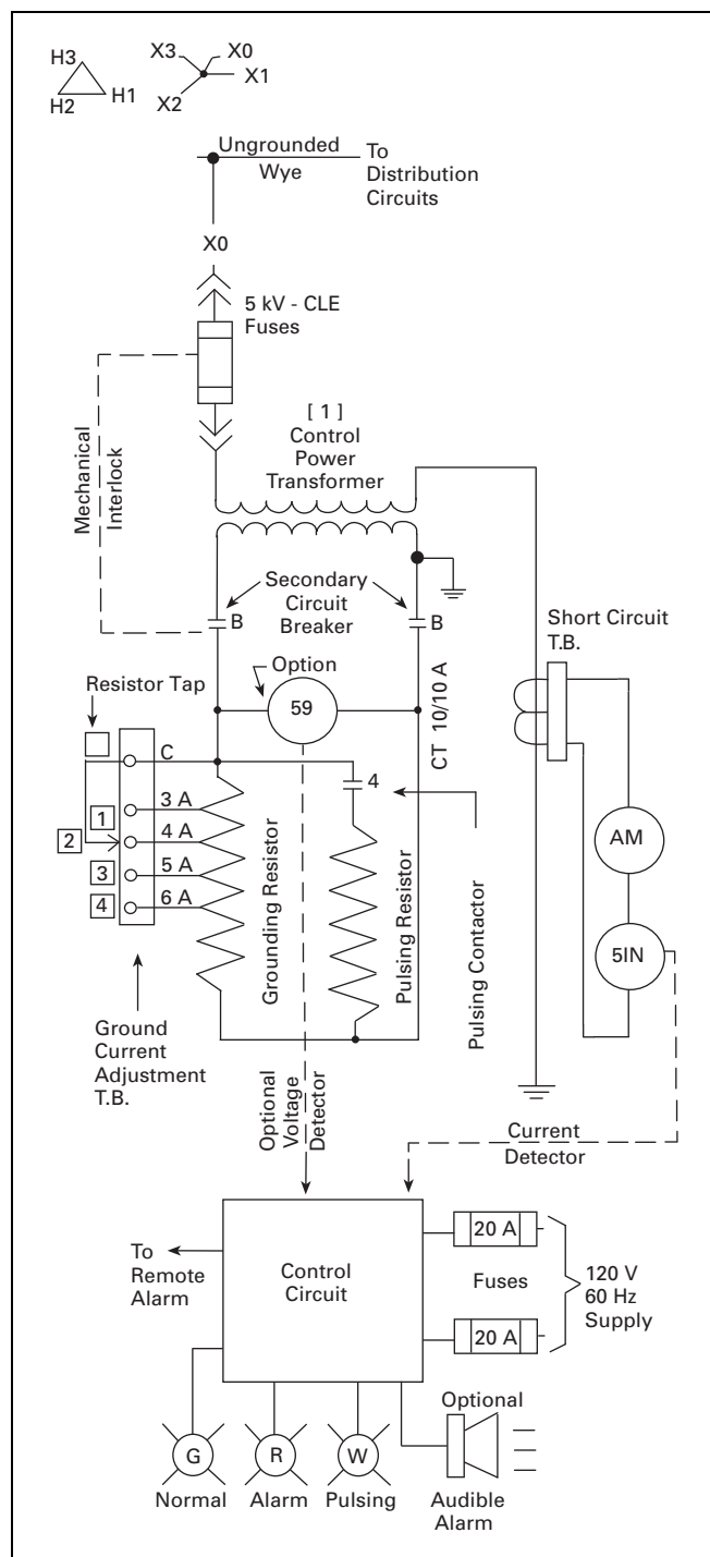
Figure 36.1-2. Ungrounded Wye System (With Standard Current and Optional Voltage Relay Fault Detectors)
