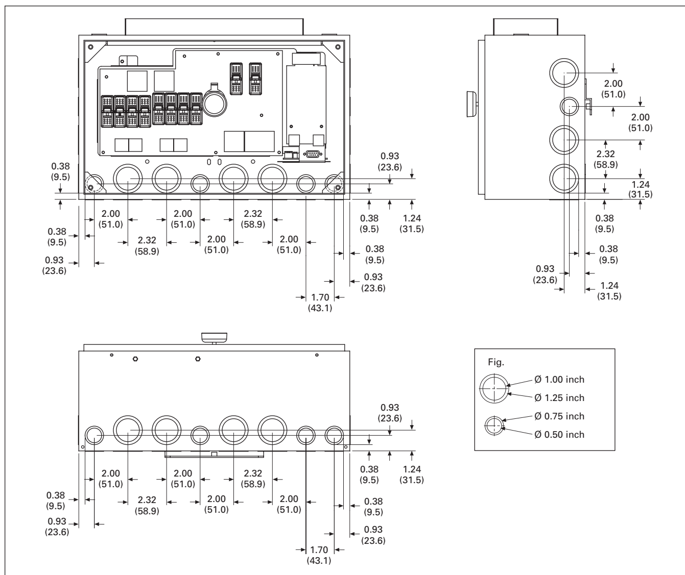
Figure 39.1-3. Knockouts on the Wiring Box
