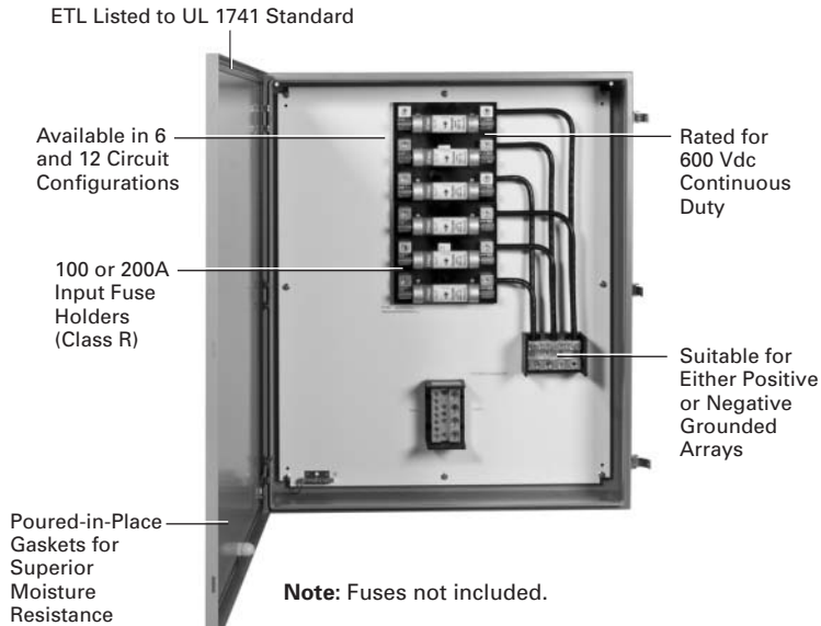
Array Combiner Features
