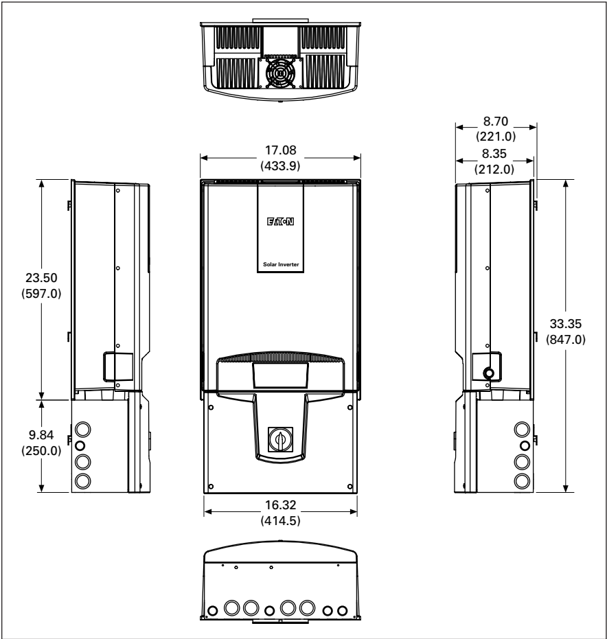
Figure 39.1-2. 3.8-7 kW Grid-Tied Solar Inverter Dimensions
