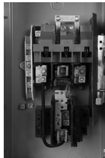
Solar Disconnect Switch (Interior View)
