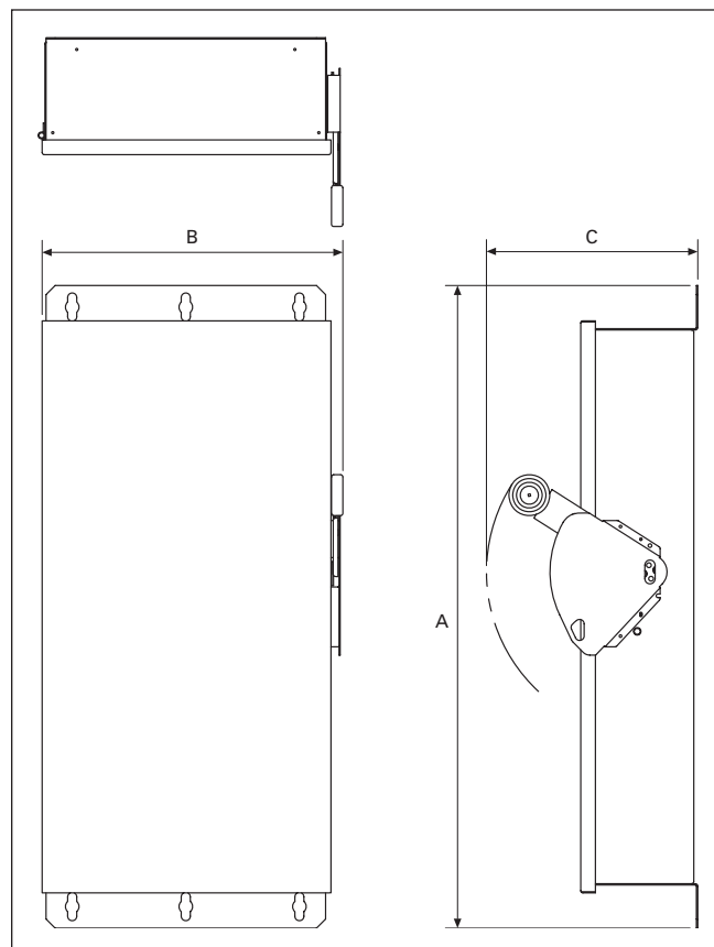
Figure 39.2-7. Type 12-3R and 4X Solar Switch Dimensions
