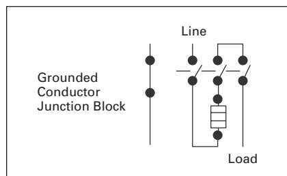
Figure 39.2-2. Fused Construction
