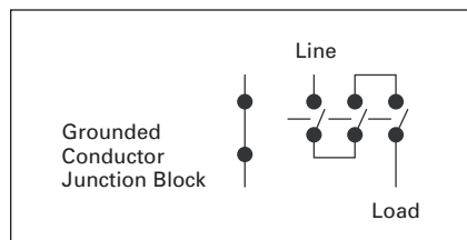
Figure 39.2-1. Non-Fused Construction
