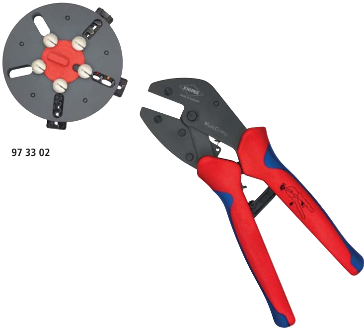
Changing the crimping dies: unlock the magazine position, take out the set of dies which the pliers have been pushed on
