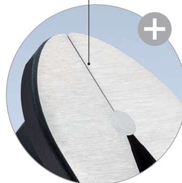
Materials are cut flush thanks to the almost bevel-free precision cutting edge
