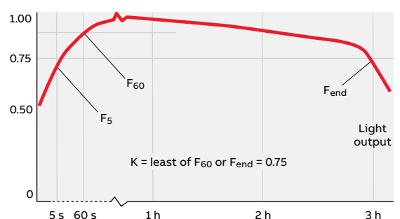
Figure 45: Service correction factors
