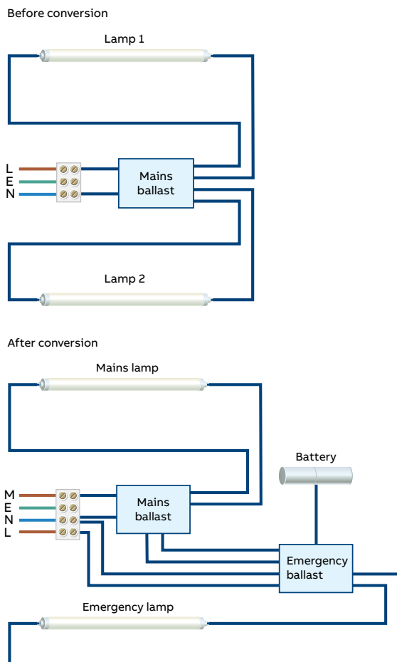
Figure 13: Schematic of a converted mains luminaire system (before and after conversion)
