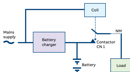
Figure 7: Maintained DC system
