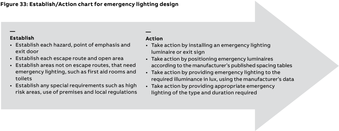
Figure 33: Establish/Action chart for emergency lighting design
