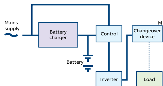
Figure 12: Maintained AC system
