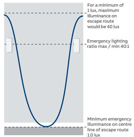
Figure 23: Uniformity requirement along escape routes
