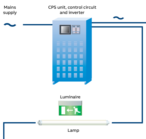
Figure 6: Schematic of a CPS system with slave emergency lighting (AC/AC system illustrated)
