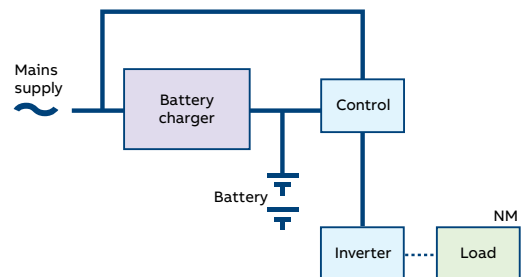
Figure 11: Non-maintained AC system
