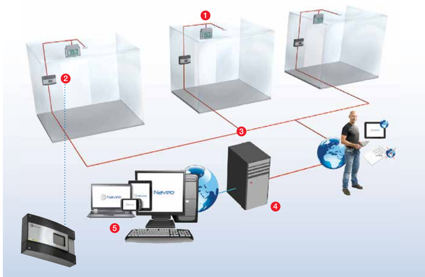
Figure 40: Emergi-Lite Naveo addressable test system with remote monitoring and management
