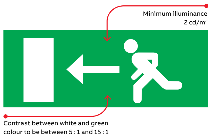
Figure 16: Exit sign formats and minimum illuminance/contrast ratios for emergency exit signs
