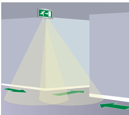
Figure 27: Providing guidance at intersections of corridors and T-junctions
