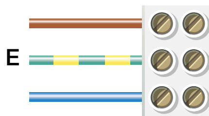
Figure 37: Wiring to slave conversion unit and central power supply
