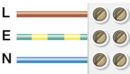
Figure 34: Non-maintained self-contained wiring
