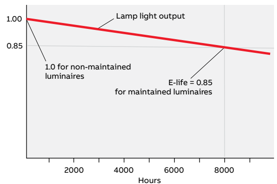
Figure 46: Maintained Factor (E-Life)
