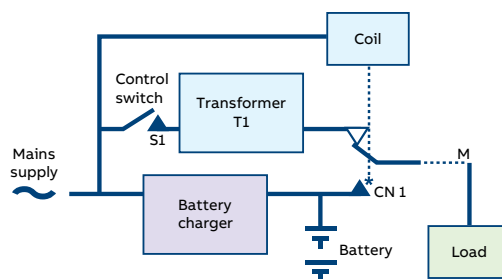
Figure 8: Maintained DC system
