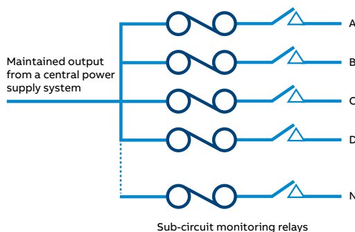
Figure 10: Maintained DC system with relays sensing each final circuit
