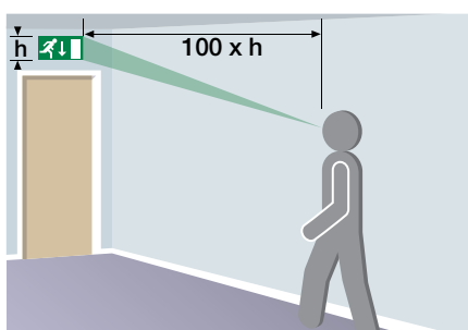
Figure 17: Viewing distance calculations for exit signboards (100 x pictogram height 'h')
