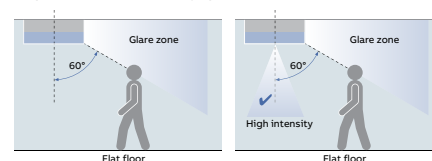
Figure 31: Disability glare at floor level
