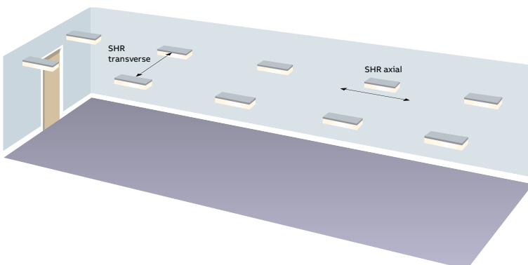
Figure 43: SHR spacing
