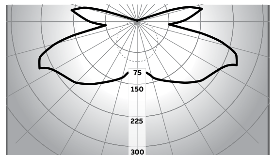
Figure 44: Luminaire relative intensity at 45 degrees
