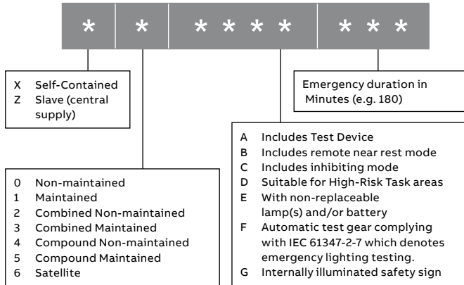
Figure 2: Labelling requirements for BS EN 60598-2-22
