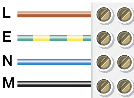
Figure 35: Maintained self-contained wiring
