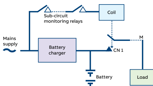
Figure 9: DC system with sub-circuit monitoring
