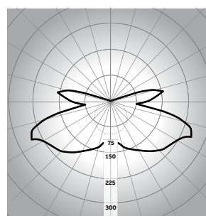
Figure 41: Luminaire relative intensity (cd/1000 lm)
