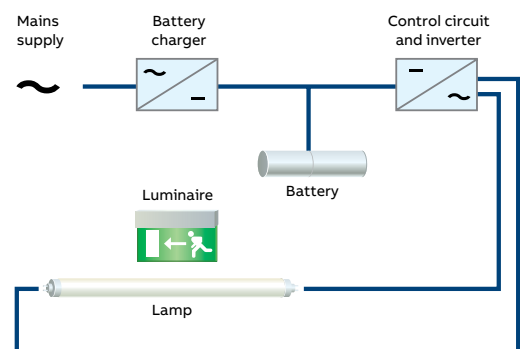
Figure 4: Schematic of a self-contained emergency luminaire
