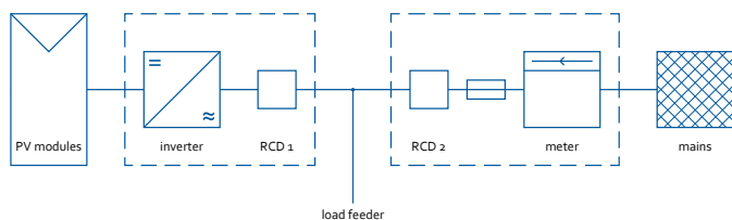
Fig. 9: Example of a system with a PV power supply system (Germany). Note UK Installations*
