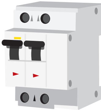
FIGURE 4 – AFDD INTEGRATED WITH AN RCBO (7.1.1 B)
