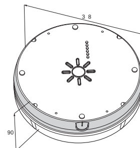
Ceiling cutout 346 mm when semi-recessing.
