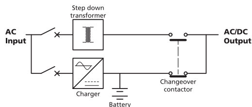
Figure 3. Central Power Supply Systems (AC/DC)
