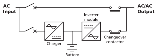
Figure 2. Static Inverter Systems (AC/AC)
