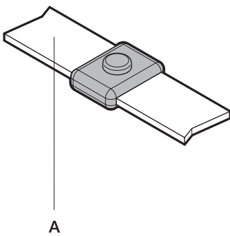
Bar to bar BB7 - FurseWELD
