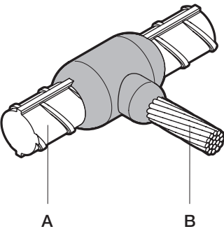
Cable to reinforcing bar CRE2 (continued) - FurseWELD
