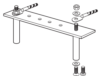
Assembly of CME kit Earth connection (not supplied)
