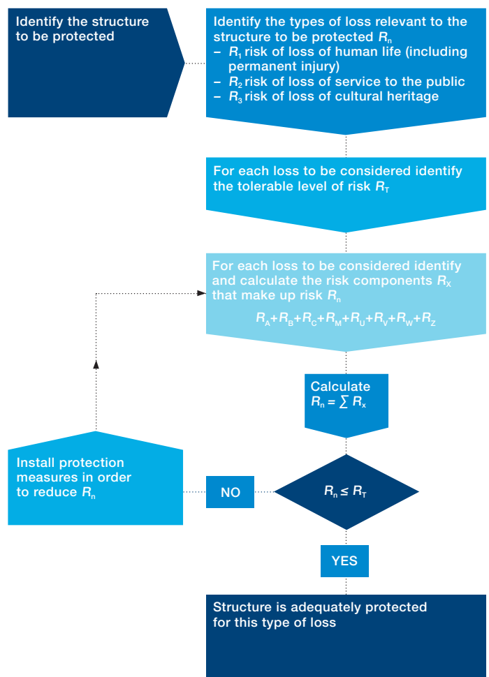
Figure 5. Procedure for deciding the need for protection (IEC/BS EN 62305-1 Figure 1)
