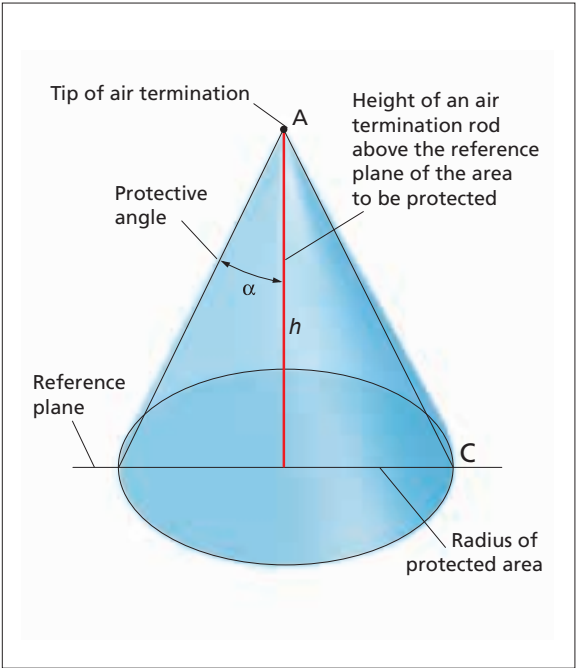
Figure 7. The protective angle method for a single air rod
