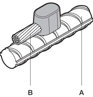
Cable to reinforcing bar CRE1 - FurseWELD
