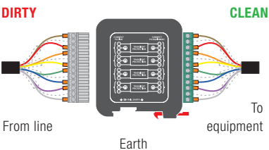
ESP RS485Q installed in series (in-line)
