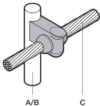
Cable to earth rod CR3 - FurseWELD
