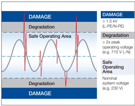
Figure 3: Equipment risk Degradation of electronic systems begins at lower transient overvoltage levels and affects critical electronic systems whenever the impulse immunity of the equipment is compromised.
