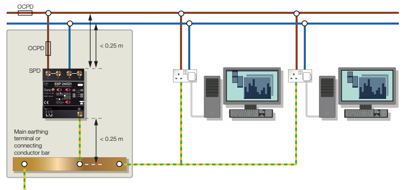
Figure 6: Critical length of connecting conductors (534.2.9)
