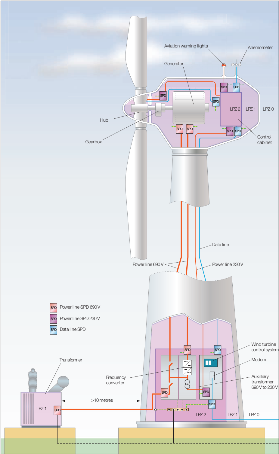
Figure 1: Application of SPDs within a typical wind turbine environment
