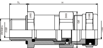
Metric Thread
