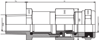
NPT Thread
