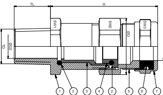
NPT Thread
