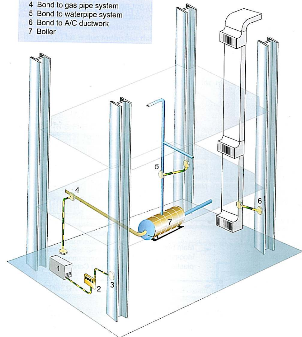
Figure E 6.4 Protective equipotential bonding – utilizing structure as protective conductor.
