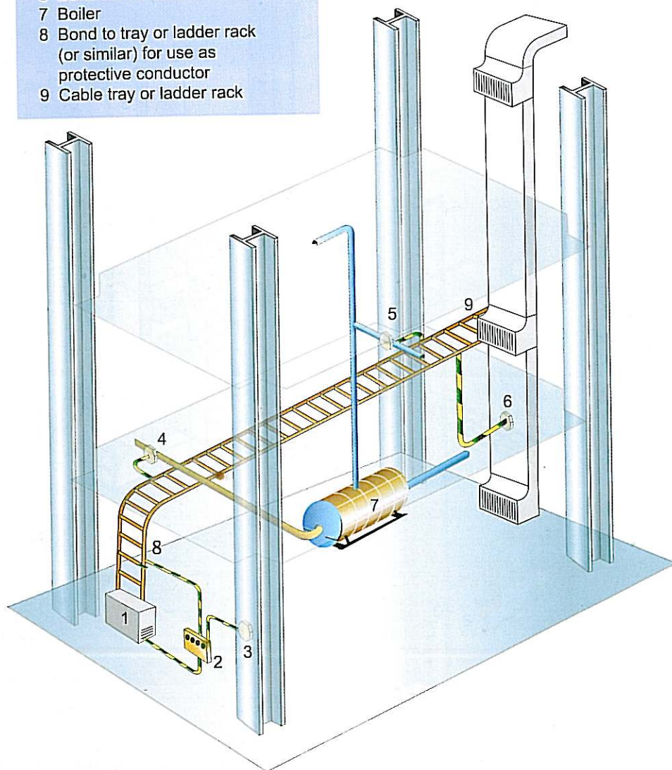
Figure E 6.3 Protective equipotential bonding – utilizing cable tray as protective conductor.
