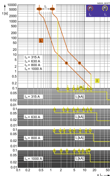
Tripping characteristics
