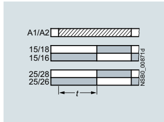
A ON-delay
