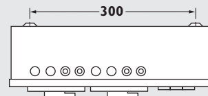
NSPE-5359/15 NSPE-5359/12 NSPE-5359/10* dimension X applies
