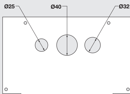
63-100A Gland Plates
