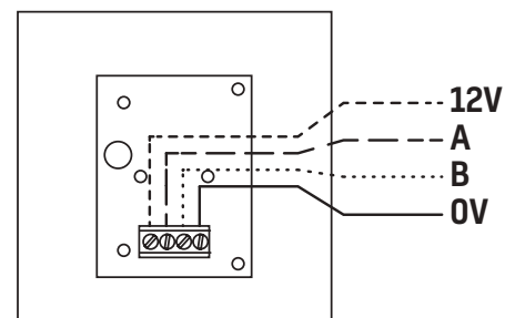
Connection at Indicator
