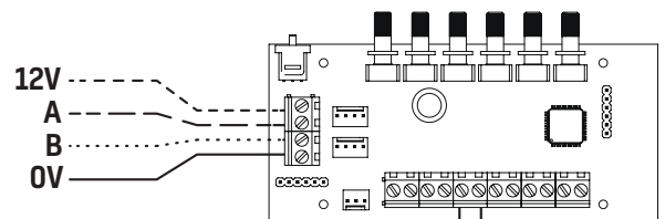
Connection at Unit
