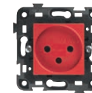
GW 34 217 Israeli Standard 2P+ E - 16A - 250V
