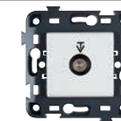
GW 34 246 - 0 dB Male IEC Ø 9.5mm (40 - 862 MHz)
