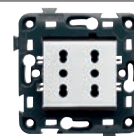
GW 34 221 Italian Standard - double 2P+ E - 10/16A 250V ac
