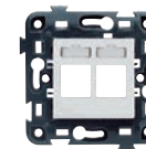
Double enclosure for RJ45 GW 34 282 for AMP GW 34 284 for AVAYA
