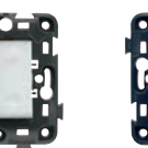
GW 34 053 Double push-button 1P - NO - 10A - 250V ac
