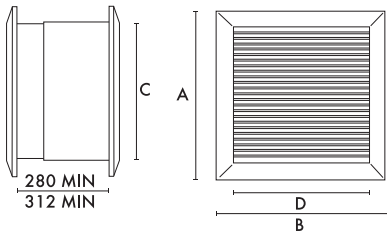
CxD SQ. HOLE THROUGH WALL
