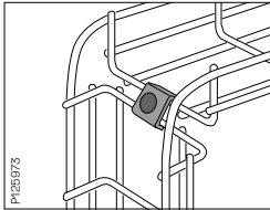
Vertical bends are joined with one or more Fitting B3, depending on mesh tray width.
