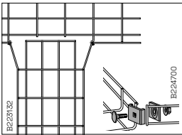
Four way and tees are joined with Fitting B3.
