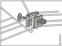
Horizontal bends are joined with Fitting B3.
