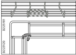
Mesh tray 53 is shaped to straight 90° angle by cutting out marked wires and joined with Fitting B3.
