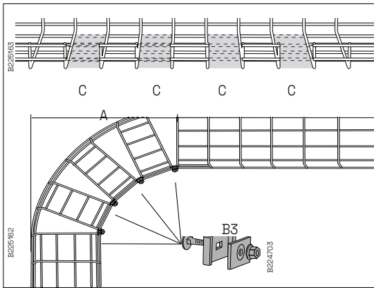
Mesh tray 120-622 is shaped to straight 90 ° angle by cutting out every other marked mesh tray section and joined with Fitting B3 according to table below.
