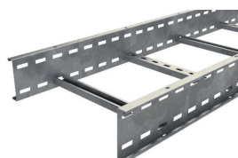
Heavy Duty Ladder 125mm high – 2mm gauge
